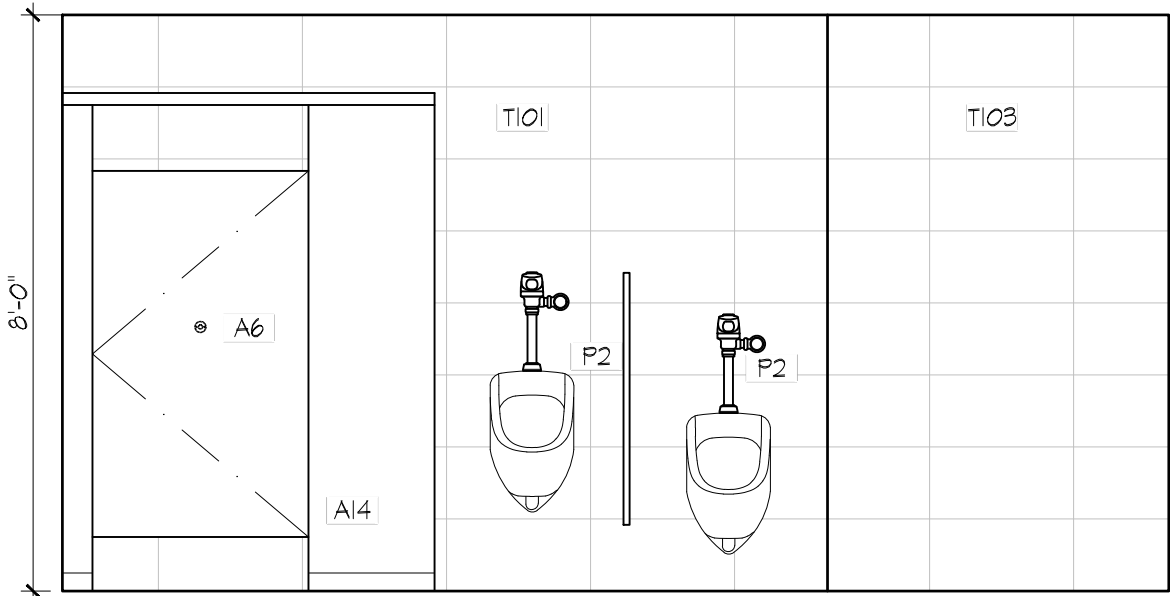
6 MEN'S 0004 NORTH 3/8" = 1'-0"
