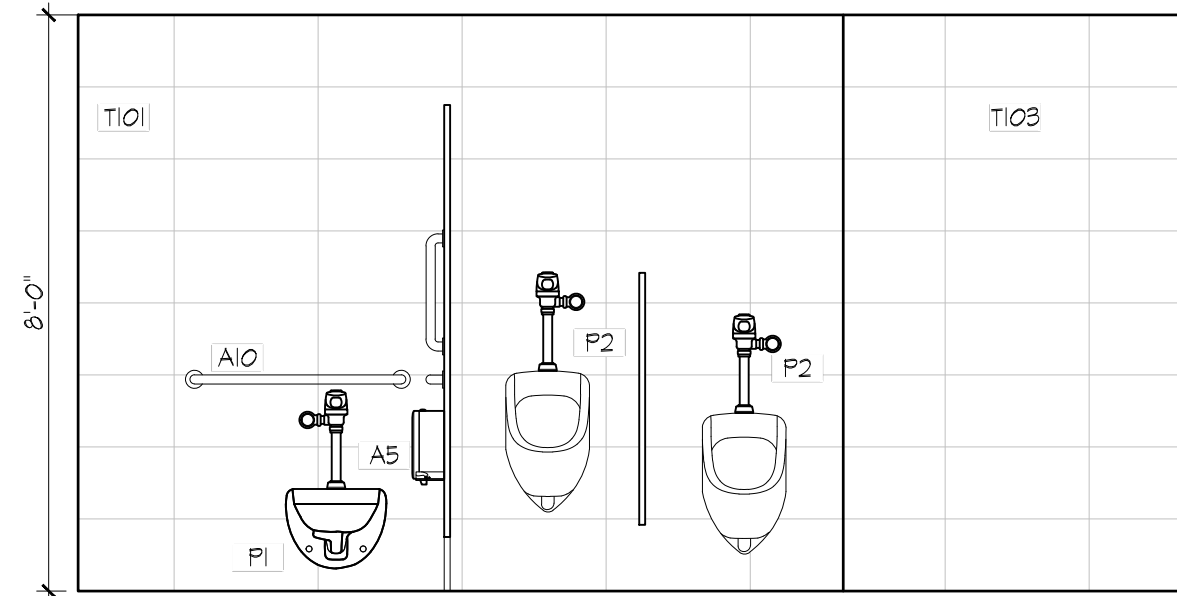
5 MEN'S 0004 NORTH 3/8" = 1'-0"
