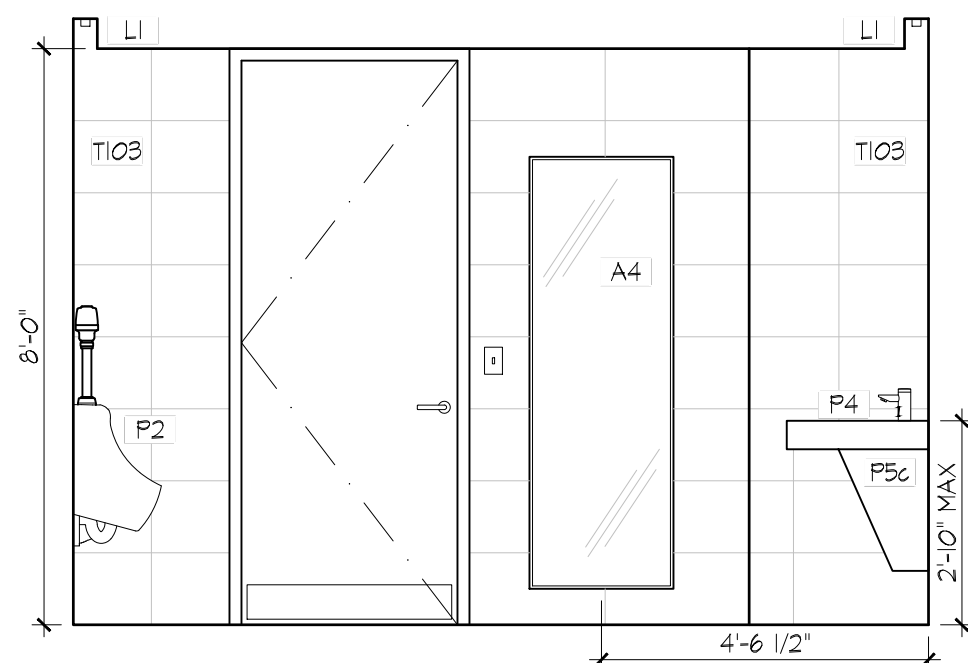
1 MEN'S 0004 EAST 3/8" = 1'-0"
