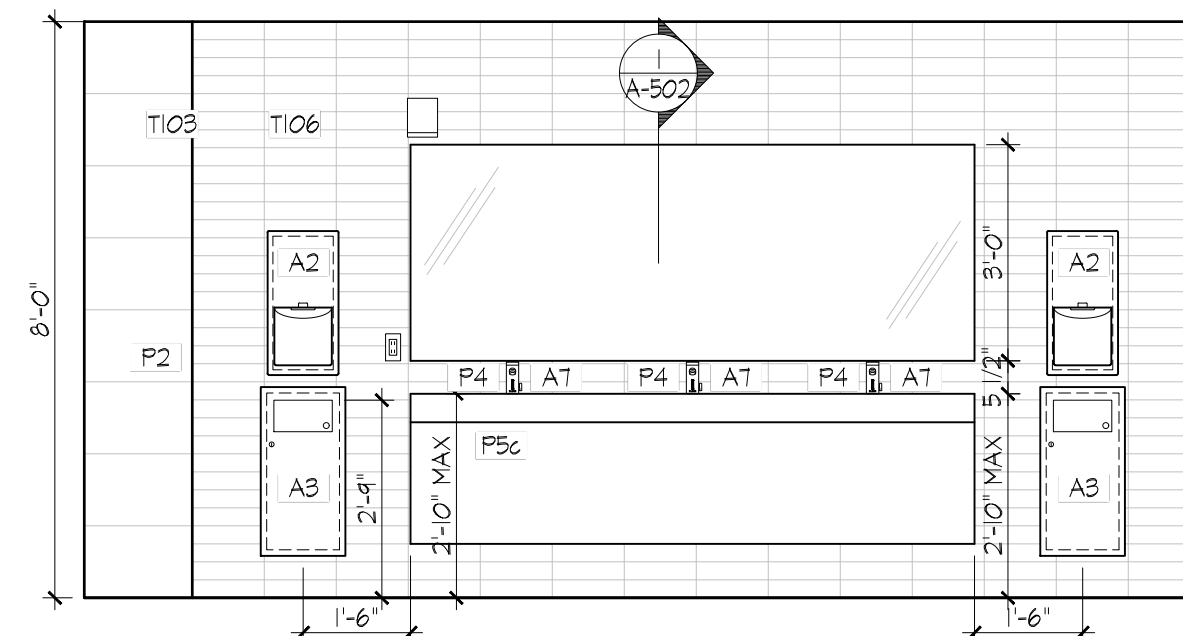
2 MEN'S 0004 SOUTH 3/8" = 1'-0"
