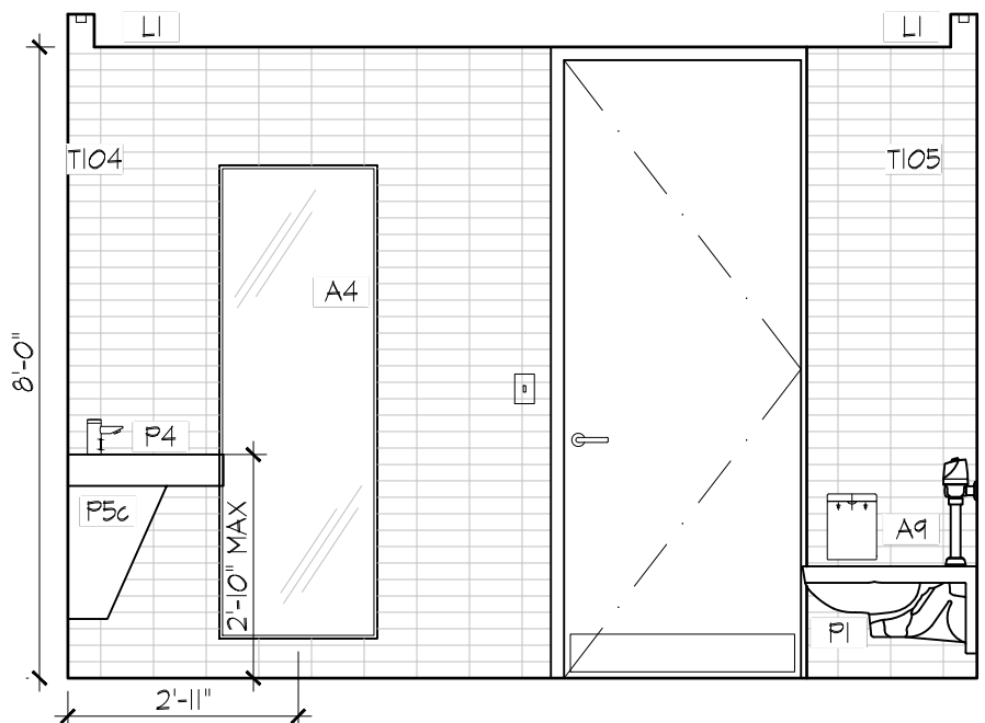
7 WOMEN'S 0004A EAST 3/8" = 1'-0"
