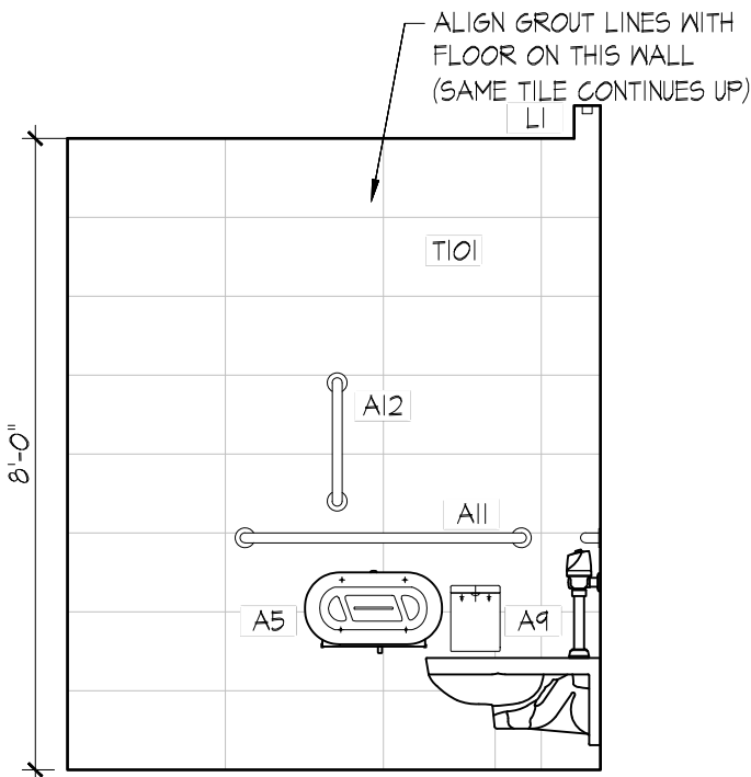
14 ALL GENDER 0004B WEST 3/8" = 1'-0"
