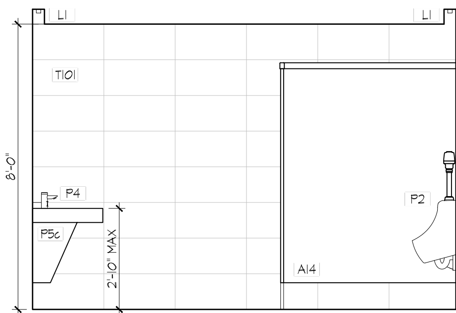
4 MEN'S 0004 WEST 3/8" = 1'-0"
