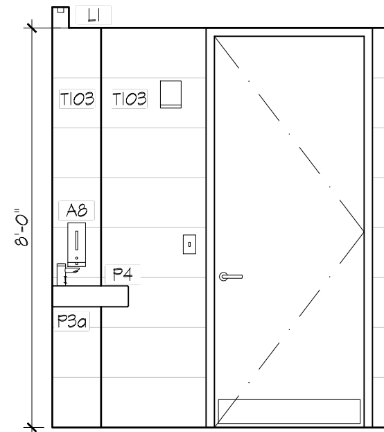
12 ALL GENDER 0004B EAST 3/8" = 1'-0"
