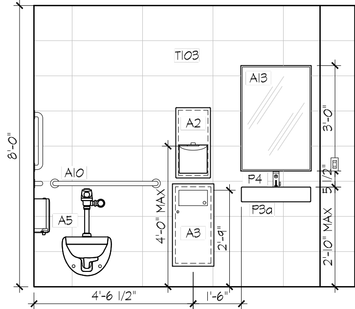
15 ALL GENDER 0004B NORTH 3/8" = 1'-0"
