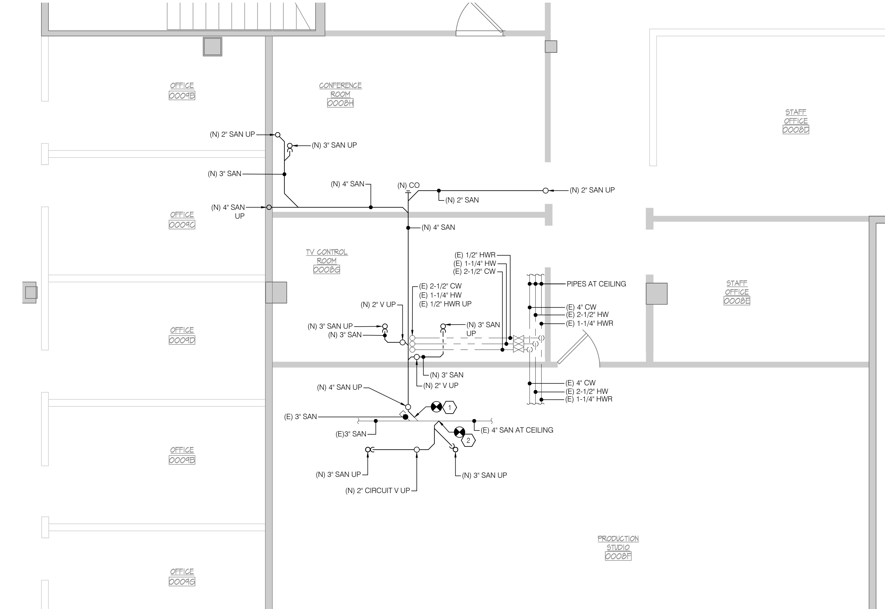
4 BASEMENT FLOOR PLAN - PLUMBING NEW WORK P-104.00 SCALE: 1/4" = 1'-0"
