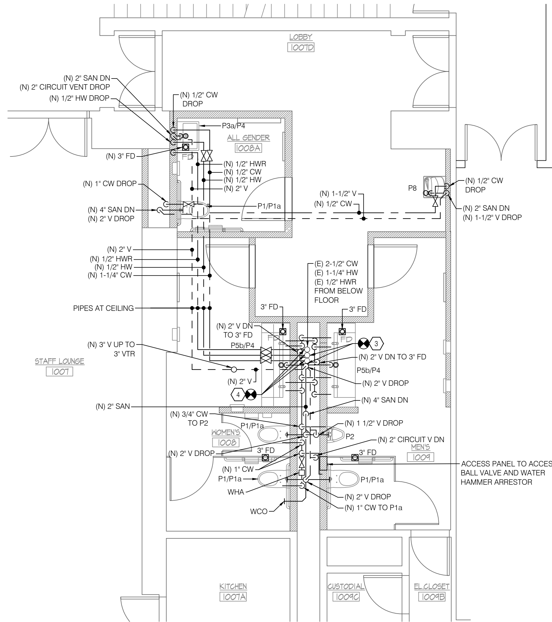
3 FIRST FLOOR PLAN PLAN - PLUMBING NEW WORK P-104.00 SCALE: 1/4" = 1'-0"
