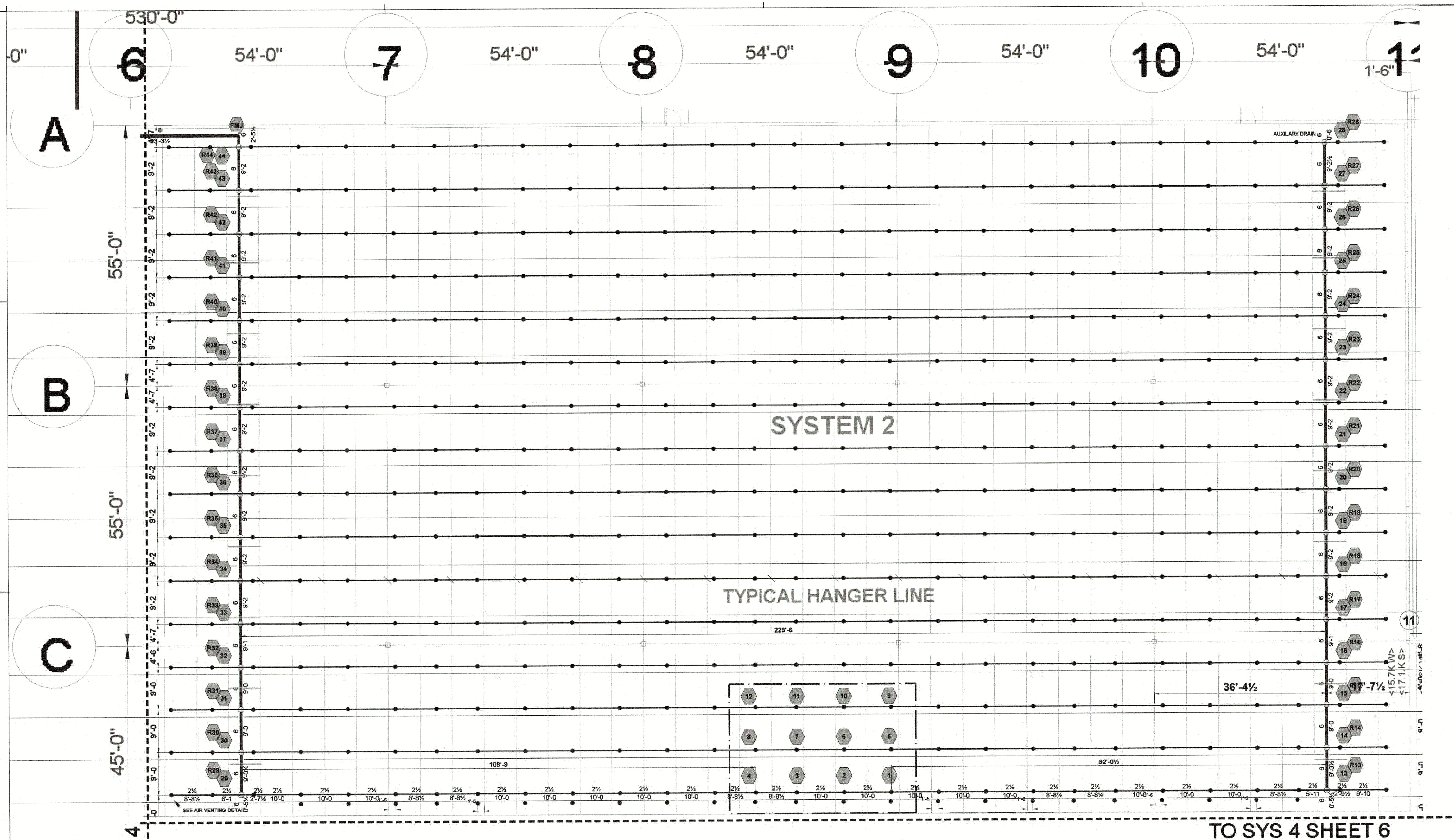
SYSTEM 2 FP PLAN 3/32 = 1'-0"
