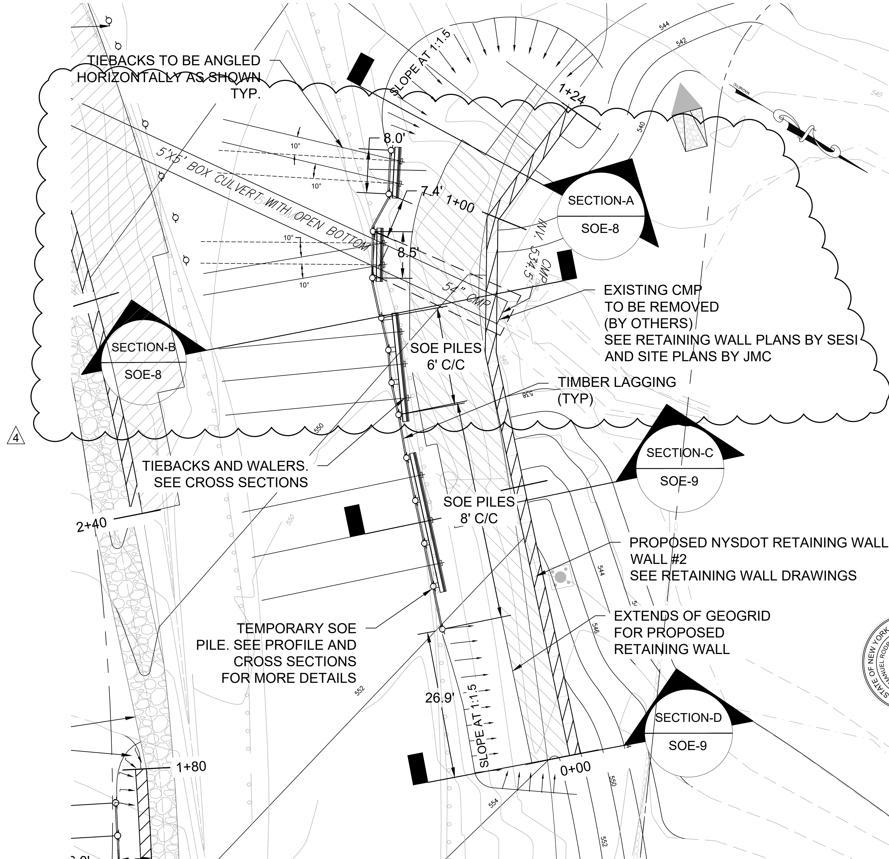
SOE WALL 2 - PLAN SCALE: 1"=10'
