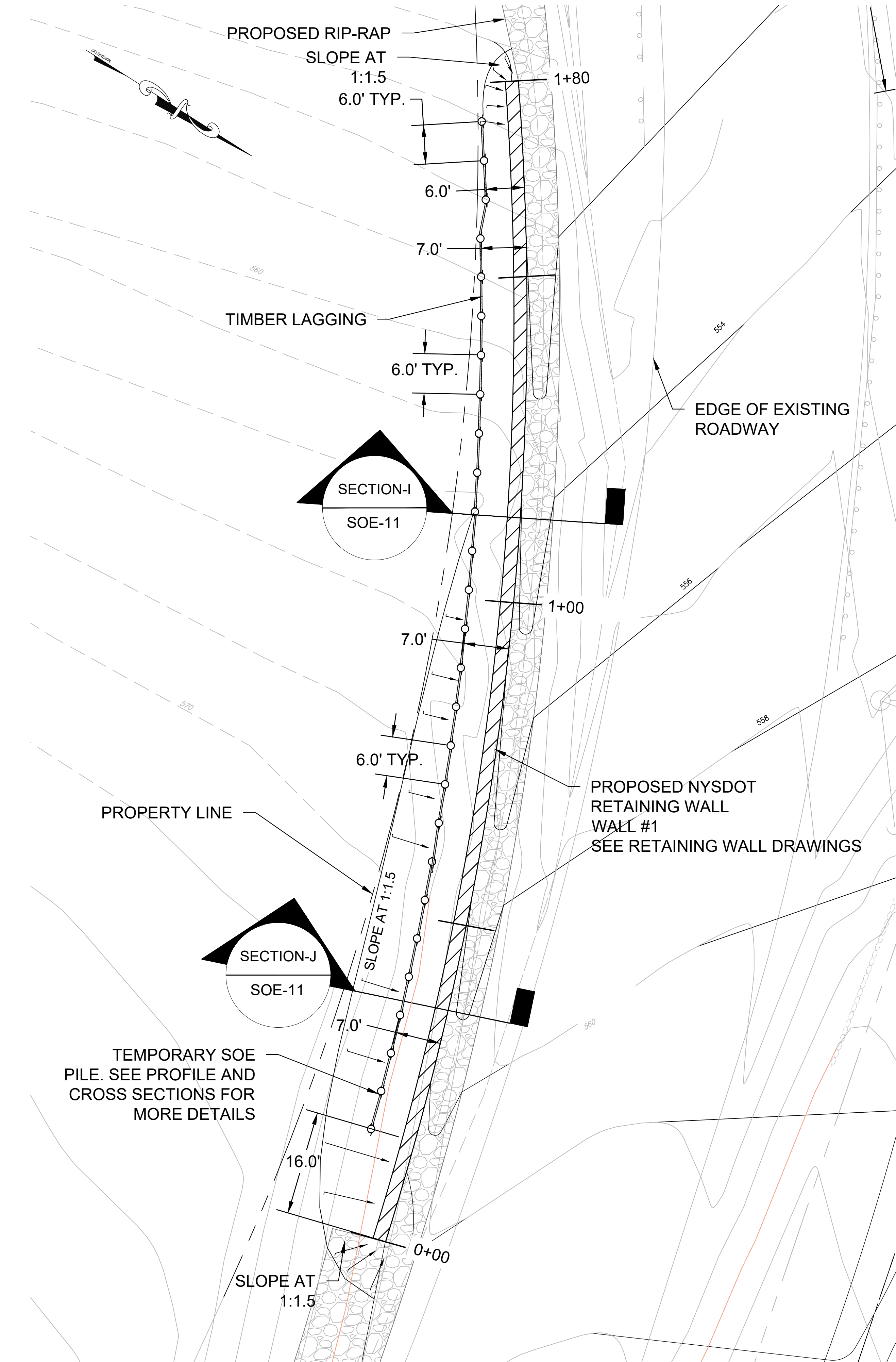
SOE WALL 1 - PLAN SCALE: 1"=10'
