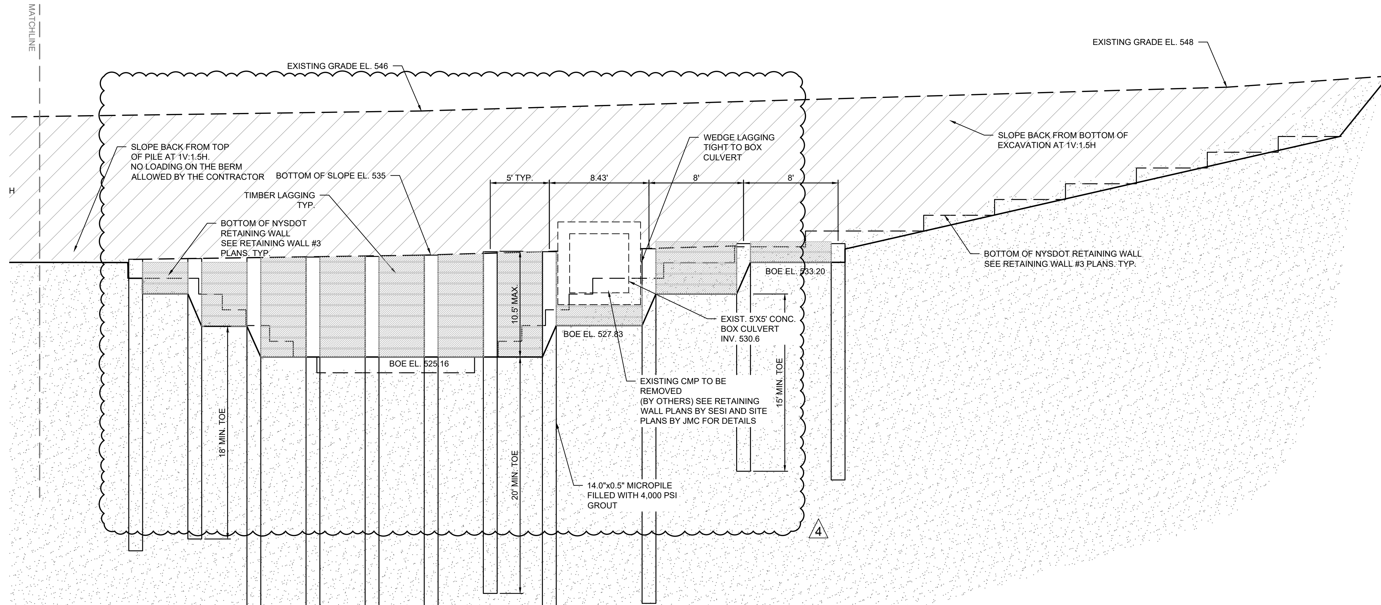
PROFILE - SOE WALL 3 SCALE 1"=5'
