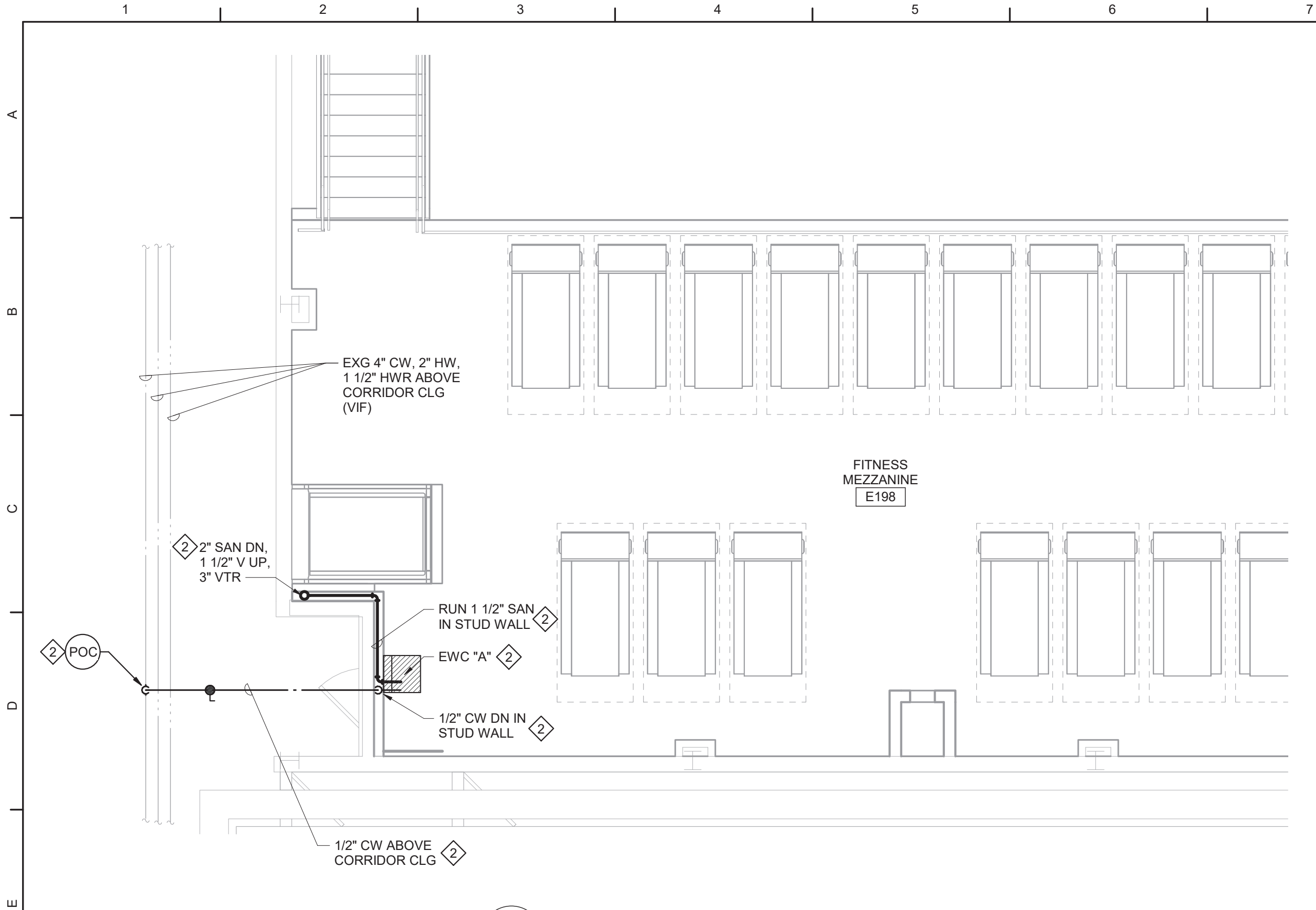
1 Partial Revised Fitness Mezzanine E198 Plan 1/4" = 1'-0"
