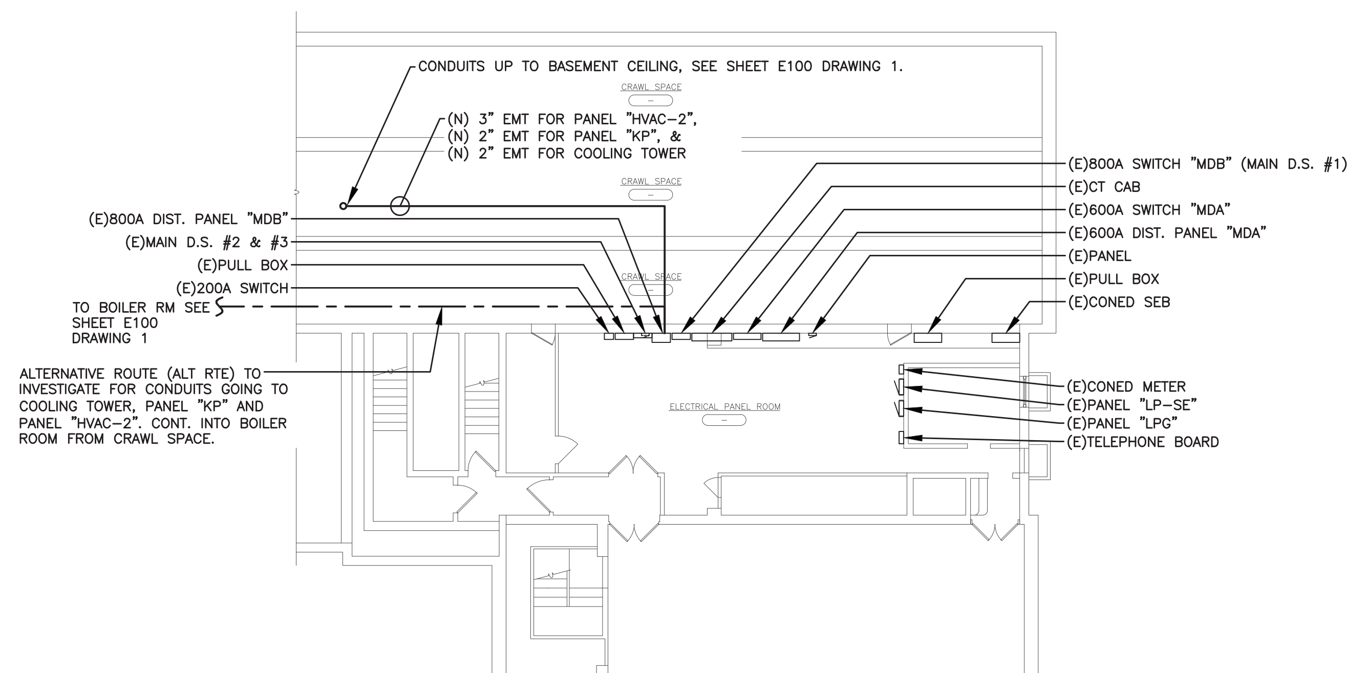
SEELY ELEMENTARY SCHOOL ELECTRICAL PLAN - SUB BASEMENT 3 SCALE: 3/32" = 1'-0"
