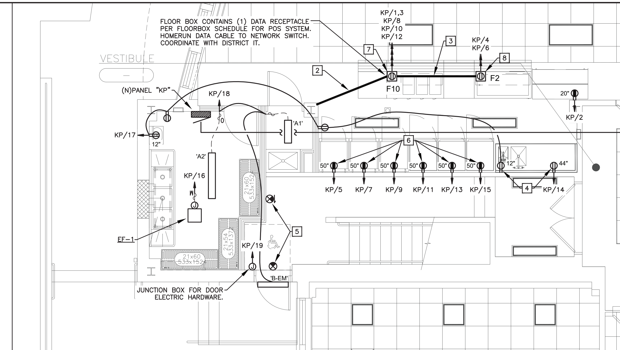
SEELY ELEMENTARY SCHOOL ENLARGED KITCHEN PLAN - LOWER LEVEL 2 SCALE: 1/4" = 1'-0"
