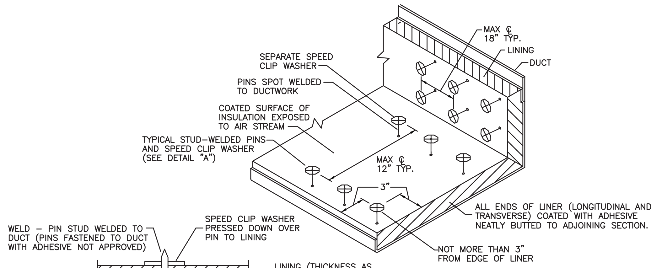
DETAIL 'A' SOUND LINING INSTALLATION DETAIL NO SCALE
