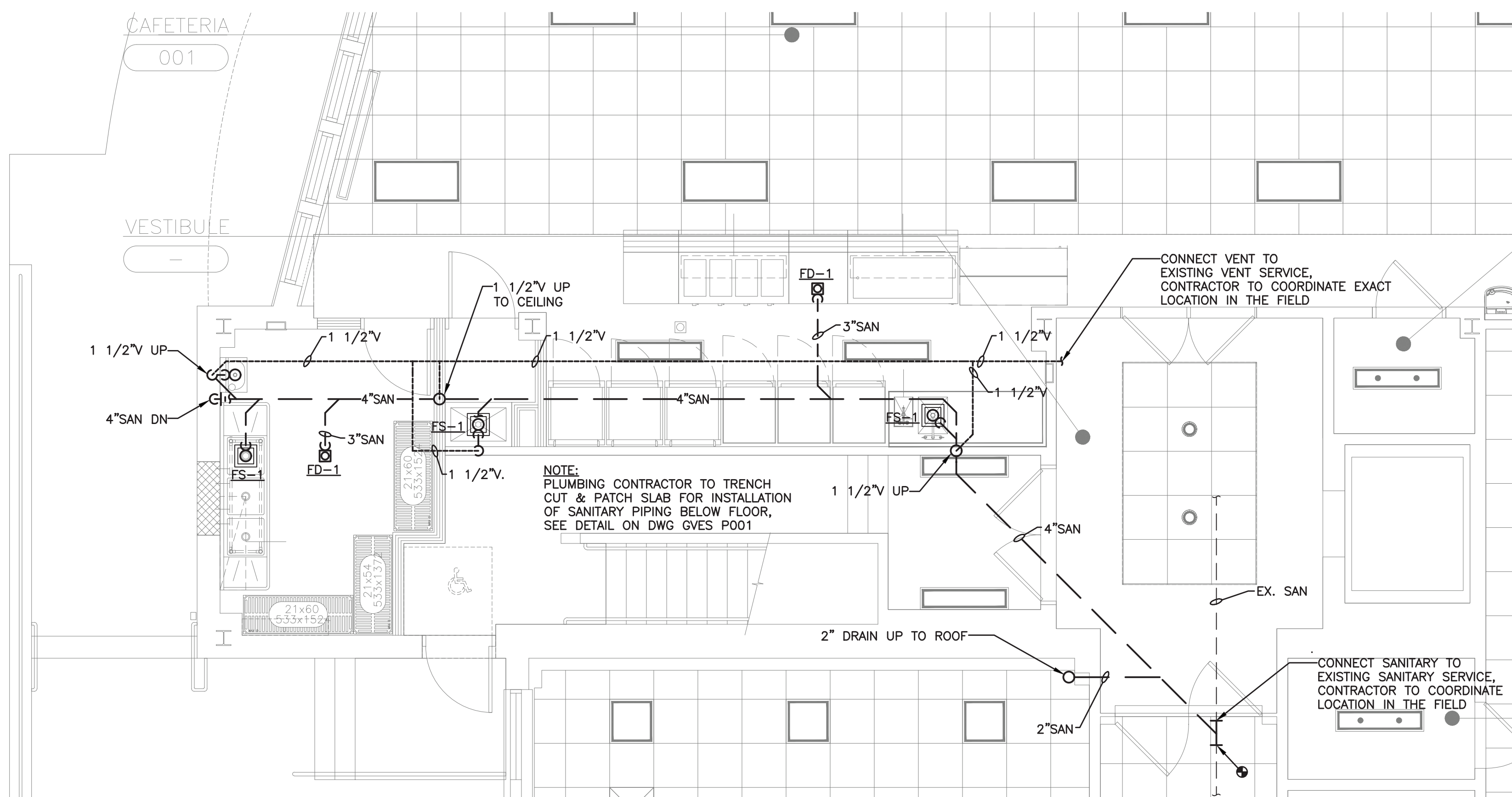
SEELY ELEMENTARY SCHOOL PART LOWER LEVEL SANITARY & VENT PLUMBING PLAN 2 SCALE: 1/4" = 1'-0"
