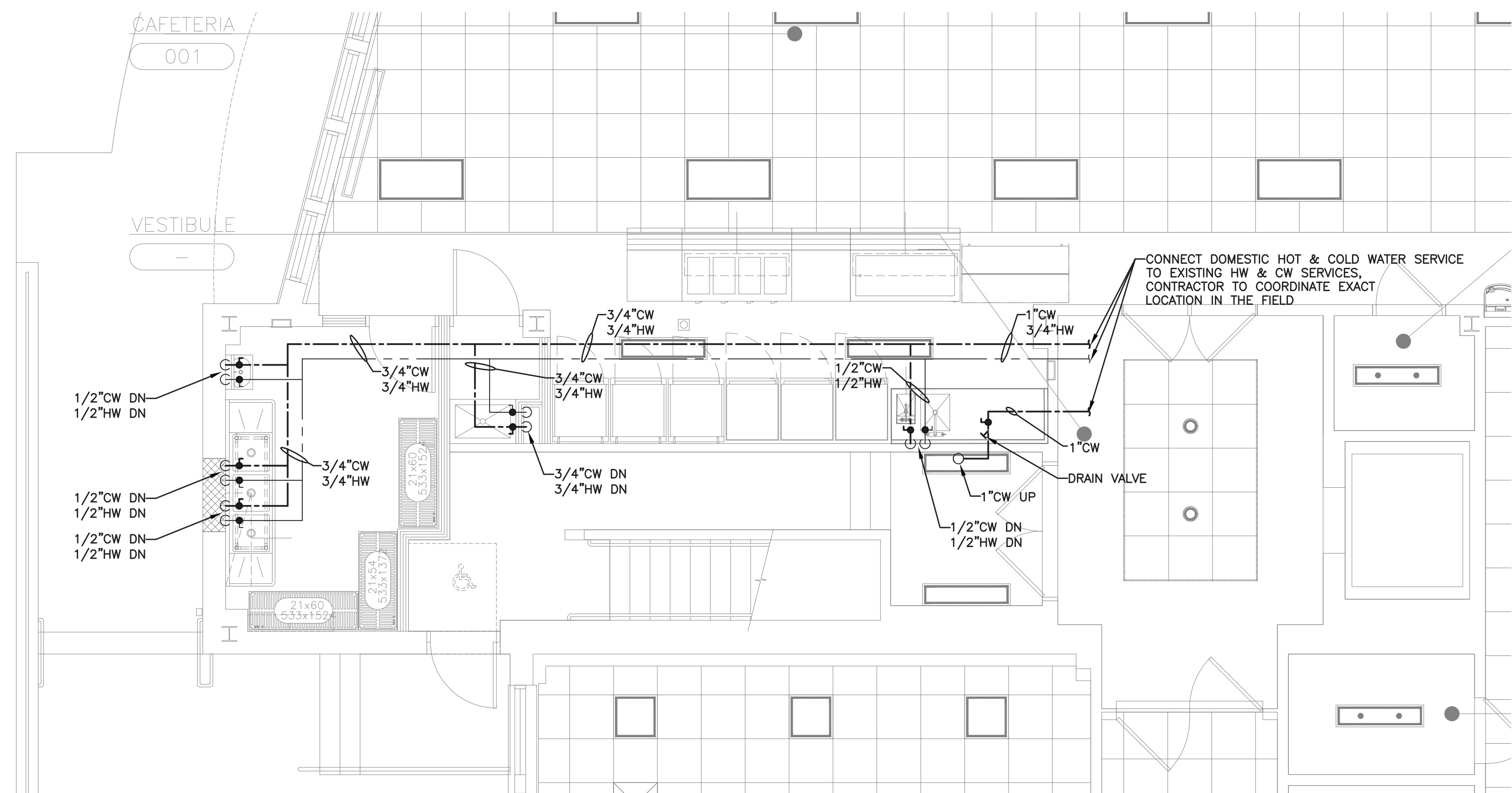
SEELY ELEMENTARY SCHOOL PART LOWER LEVEL DOMESTIC WATER PLUMBING PLAN 3 SCALE: 1/4" = 1'-0"
