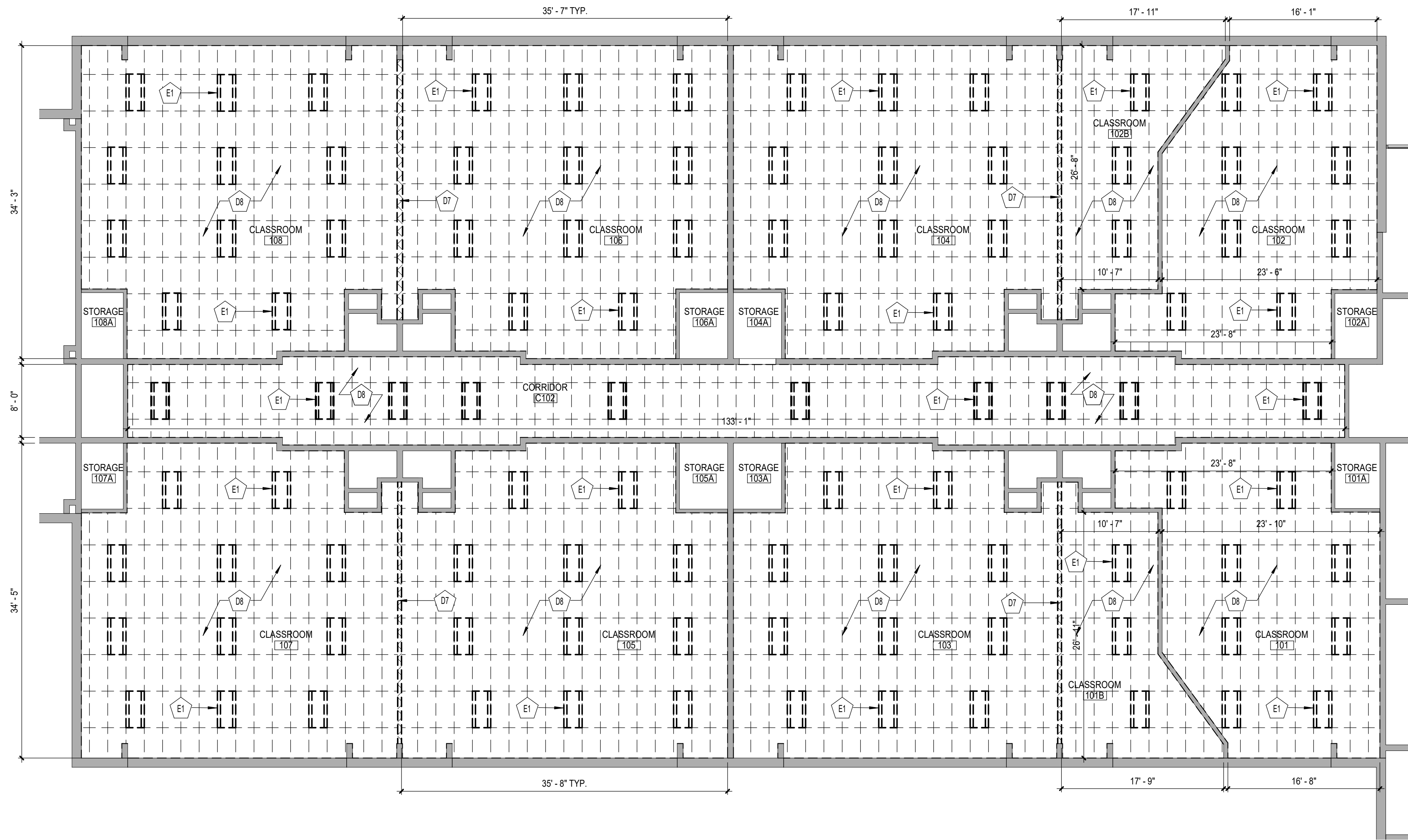
1 FIRST FLOOR DEMOLITION RCP - AREA 'B' AD812 1/8" = 1'-0"
