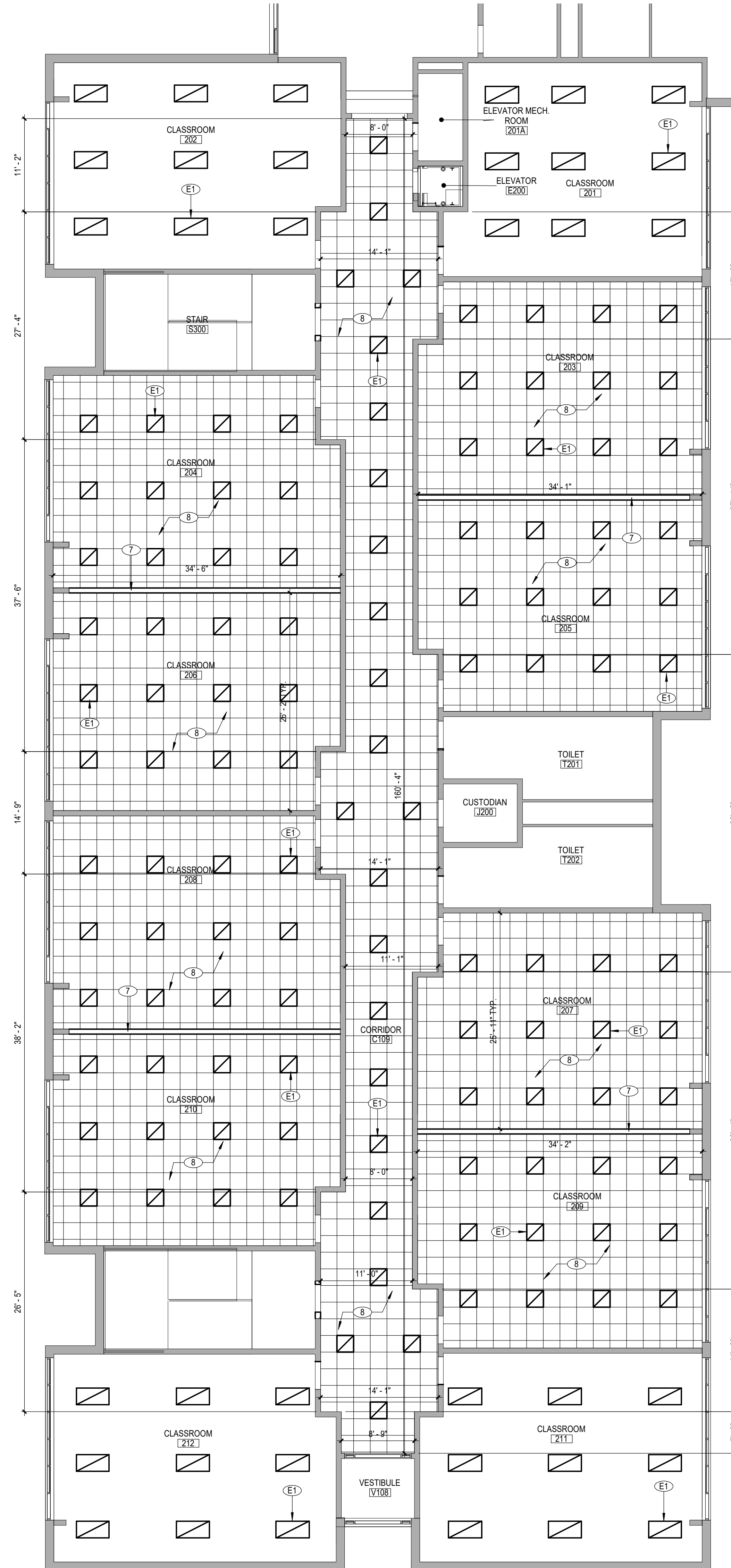
1 FIRST FLOOR NEW WORK RCP - AREA 'E' A815 1/8" = 1'-0"
