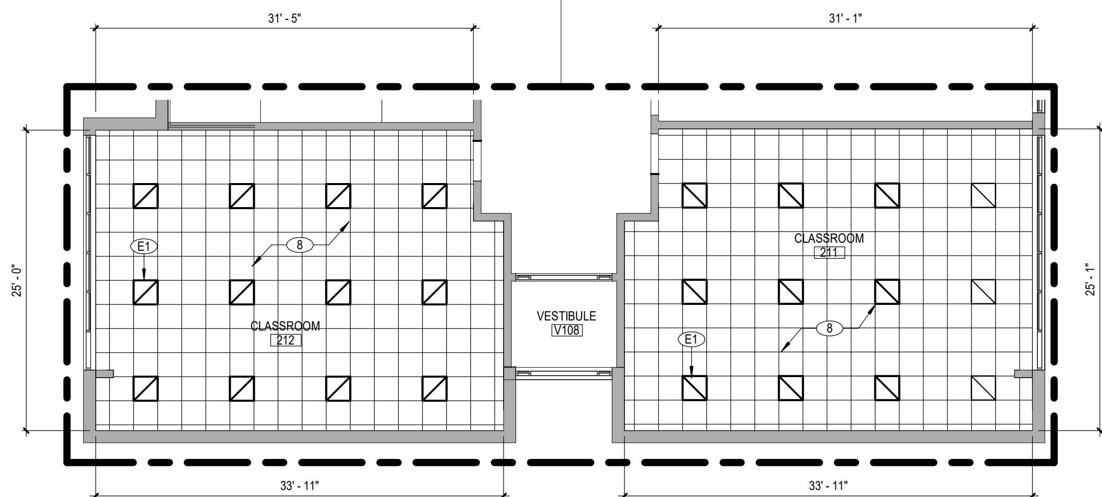
2 FIRST FLOOR NEW WORK RCP - AREA 'E' - ALTERNATE A815 1/8" = 1'-0"
