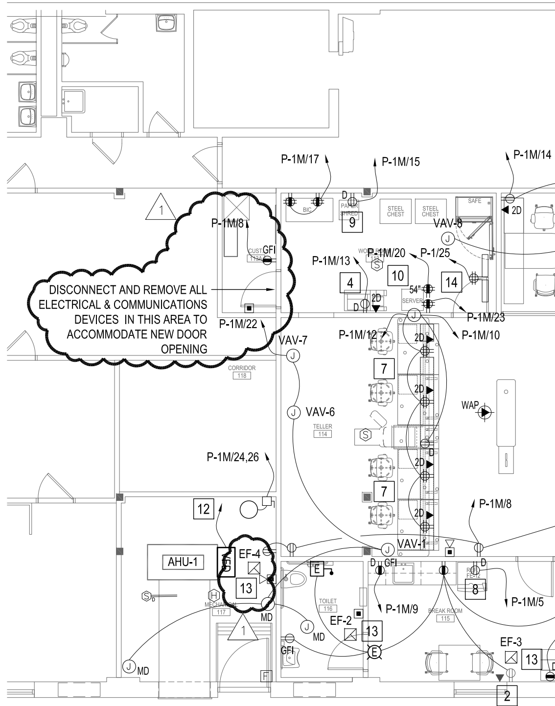
1 PART PLANS: POWER & LIGHTING SCALE: 1/8"=1'-0"
