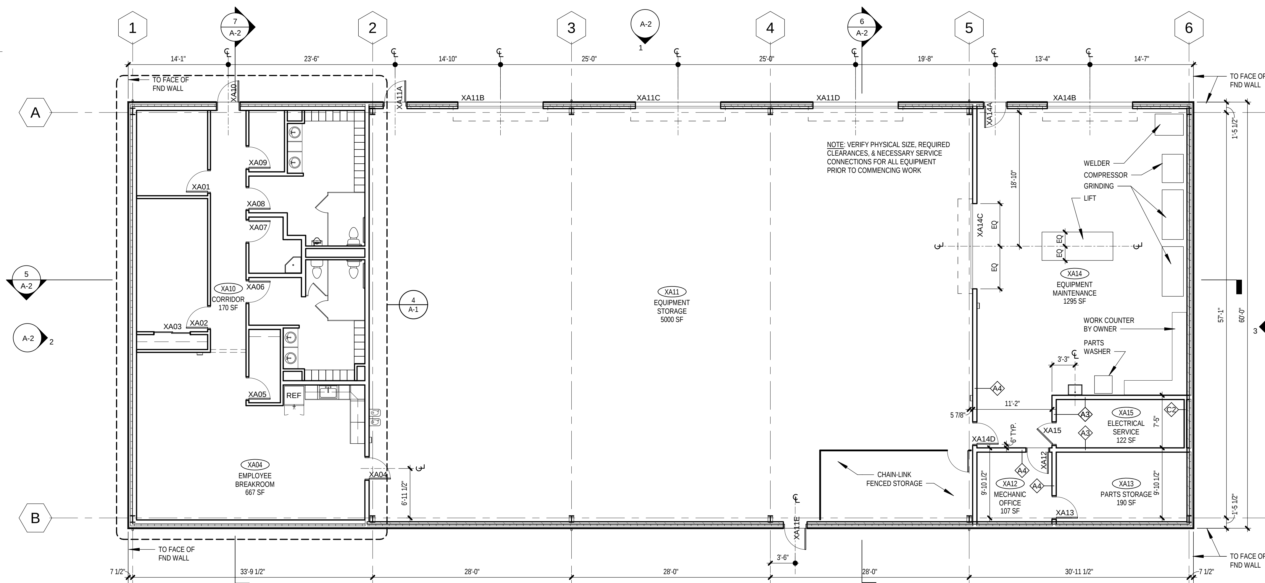
1 MAINTENANCE BUILDING - FIRST FLOOR PLAN 1/8" = 1'-0"
