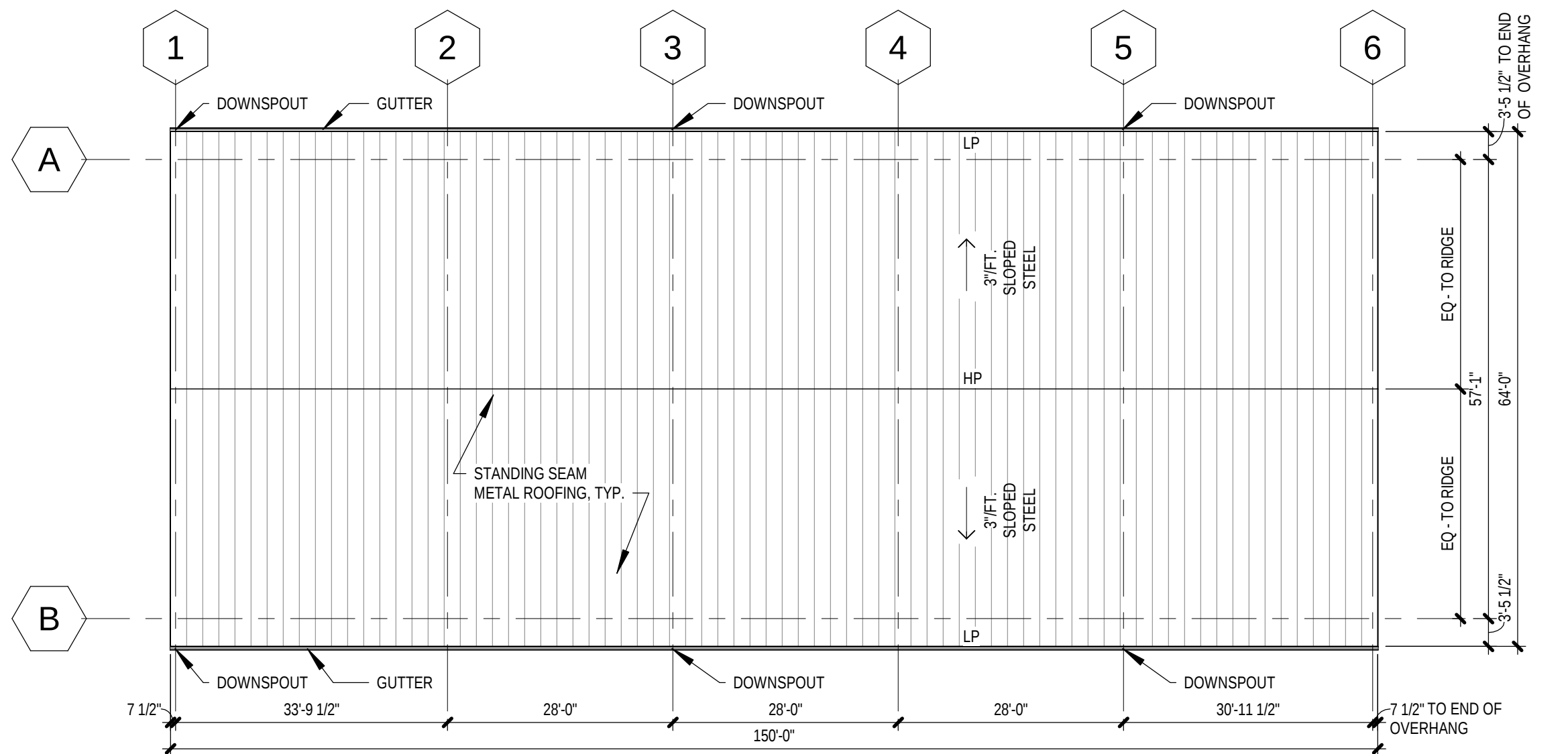
3 MAINTENANCE BUILDING - ROOF PLAN 1/16" = 1'-0"
