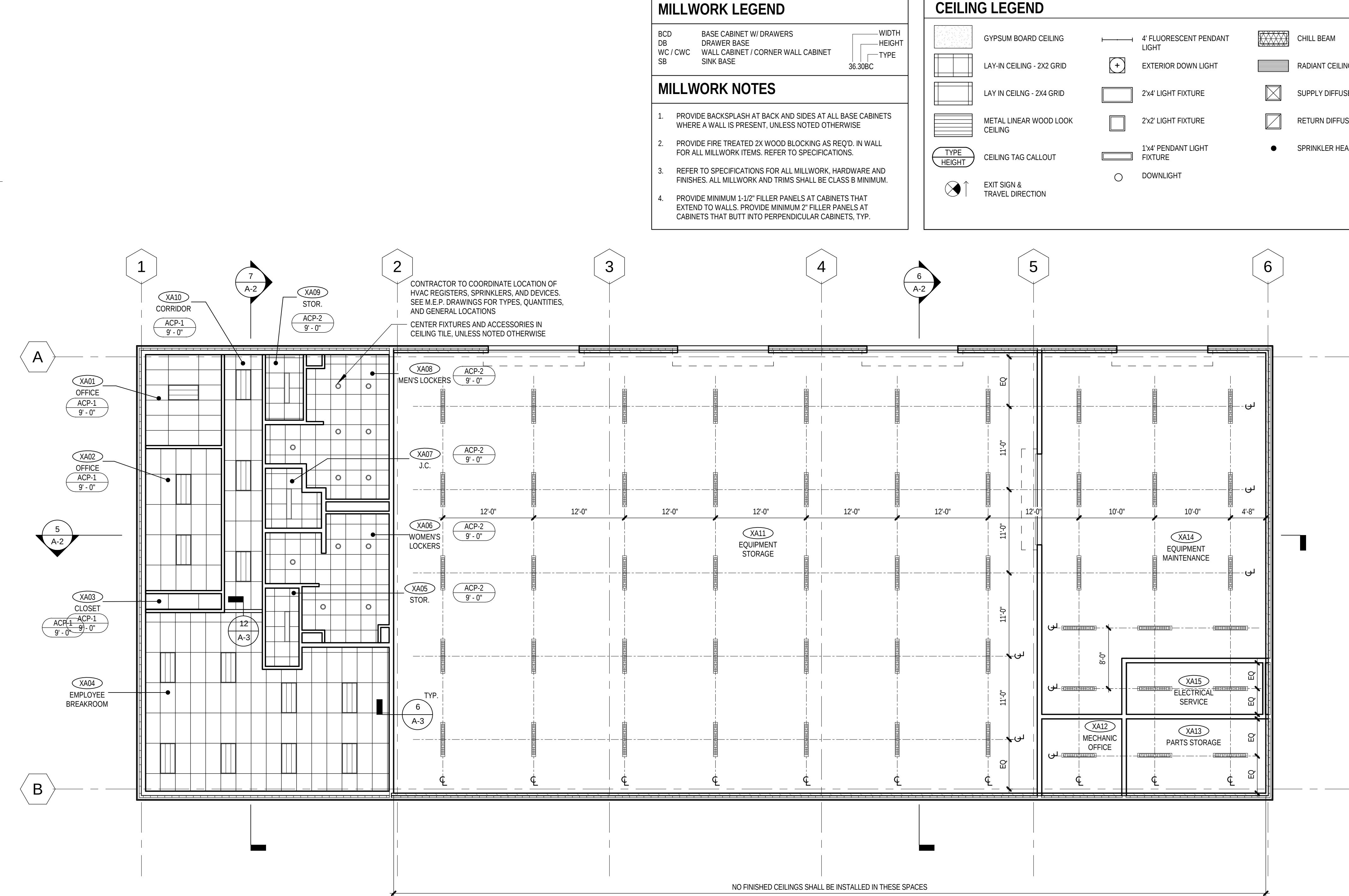
2 MAINTENANCE BUILDING - REFLECTED CEILING PLAN 1/8" = 1'-0"
