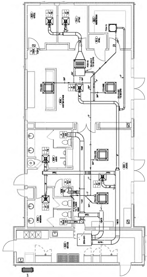
CLUBHOUSE BUILDING - FIRST FLOOR PLAN - HVAC
