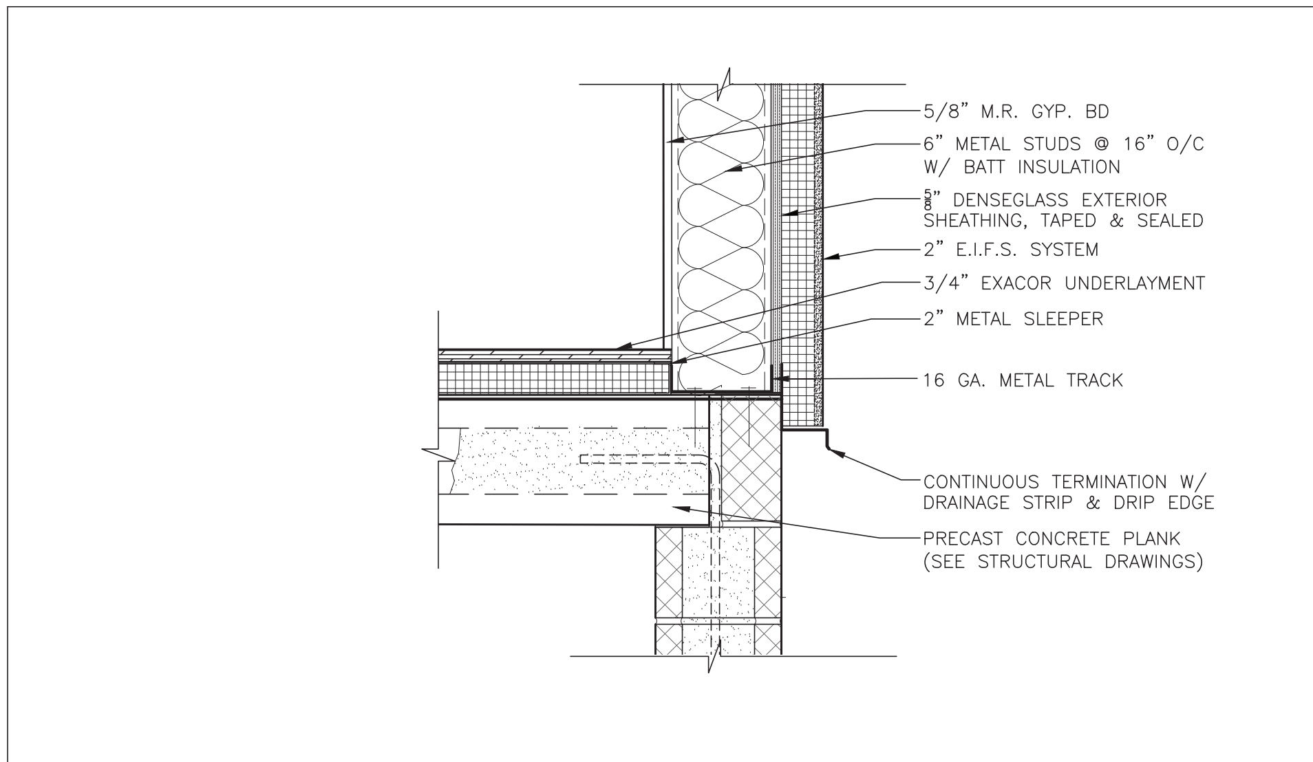
5 PRESS BOX BASE DETAIL @ BLEACHER SIDE SCALE: 1-1/2"=1'-0"
