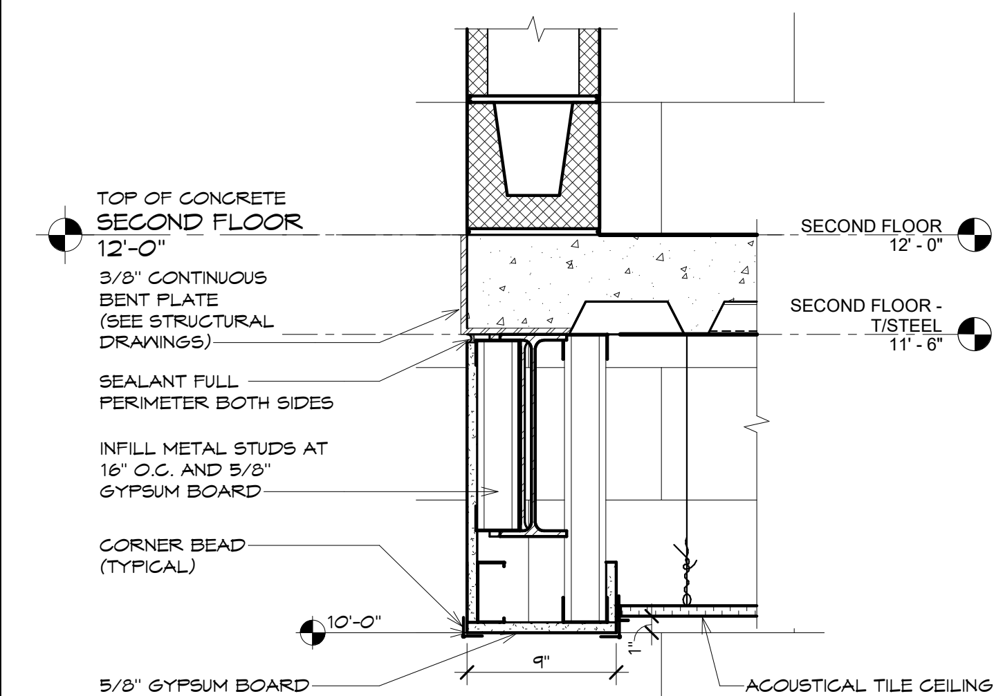
2 A400 1 1/2" = 1'-0" SOFFIT AT STAIRS
