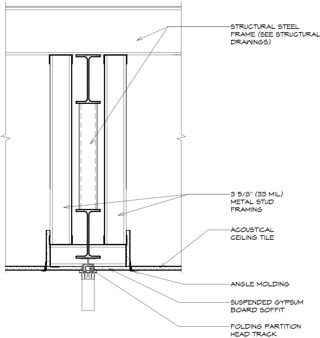
2 DETAIL A401 1 1/2" = 1'-0" GYPSUM BOARD SOFFIT AT COMMUNITY ROOM
