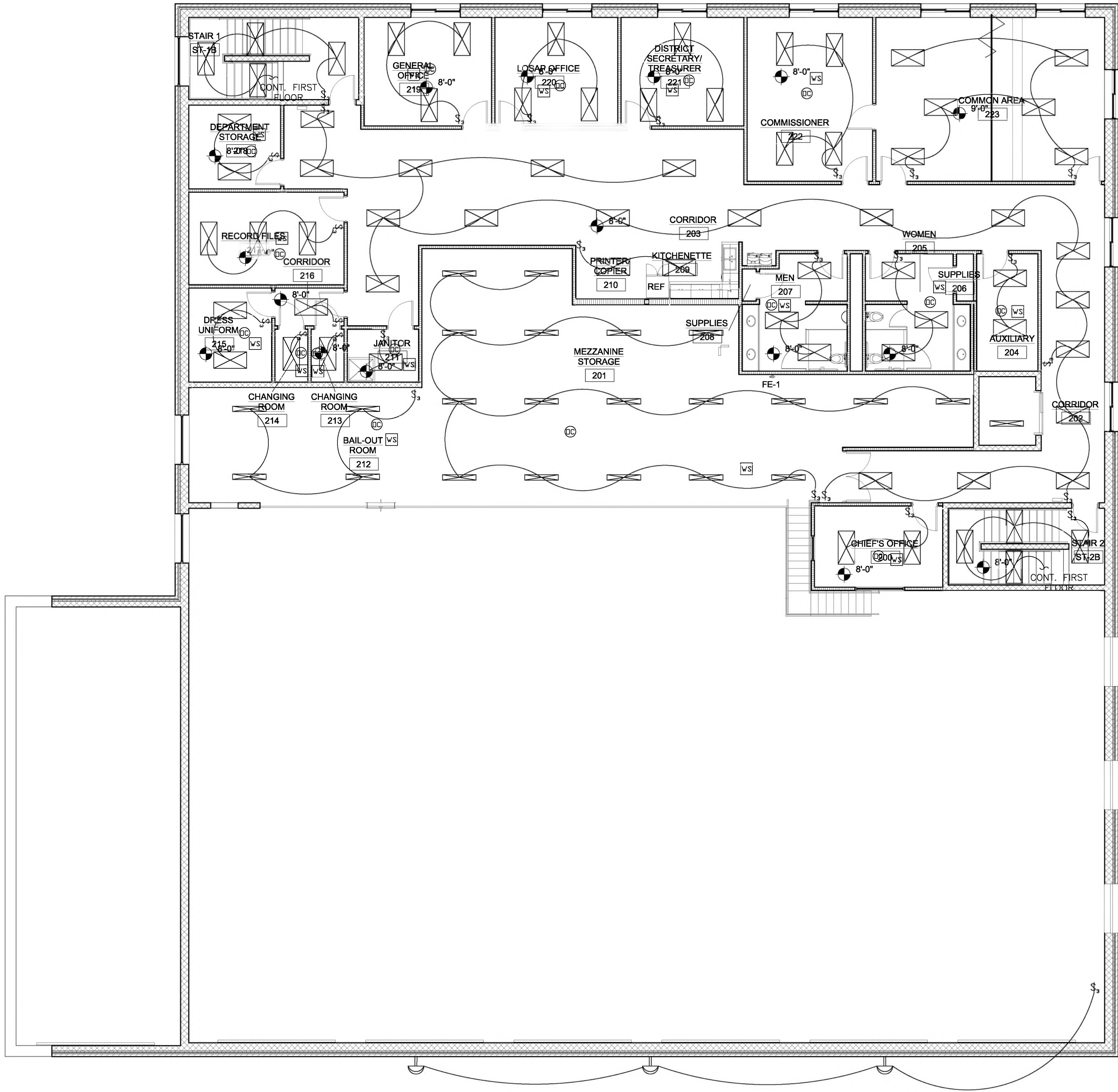
SECOND FLOOR LIGHTING PLAN 1/8" = 1'-0"
