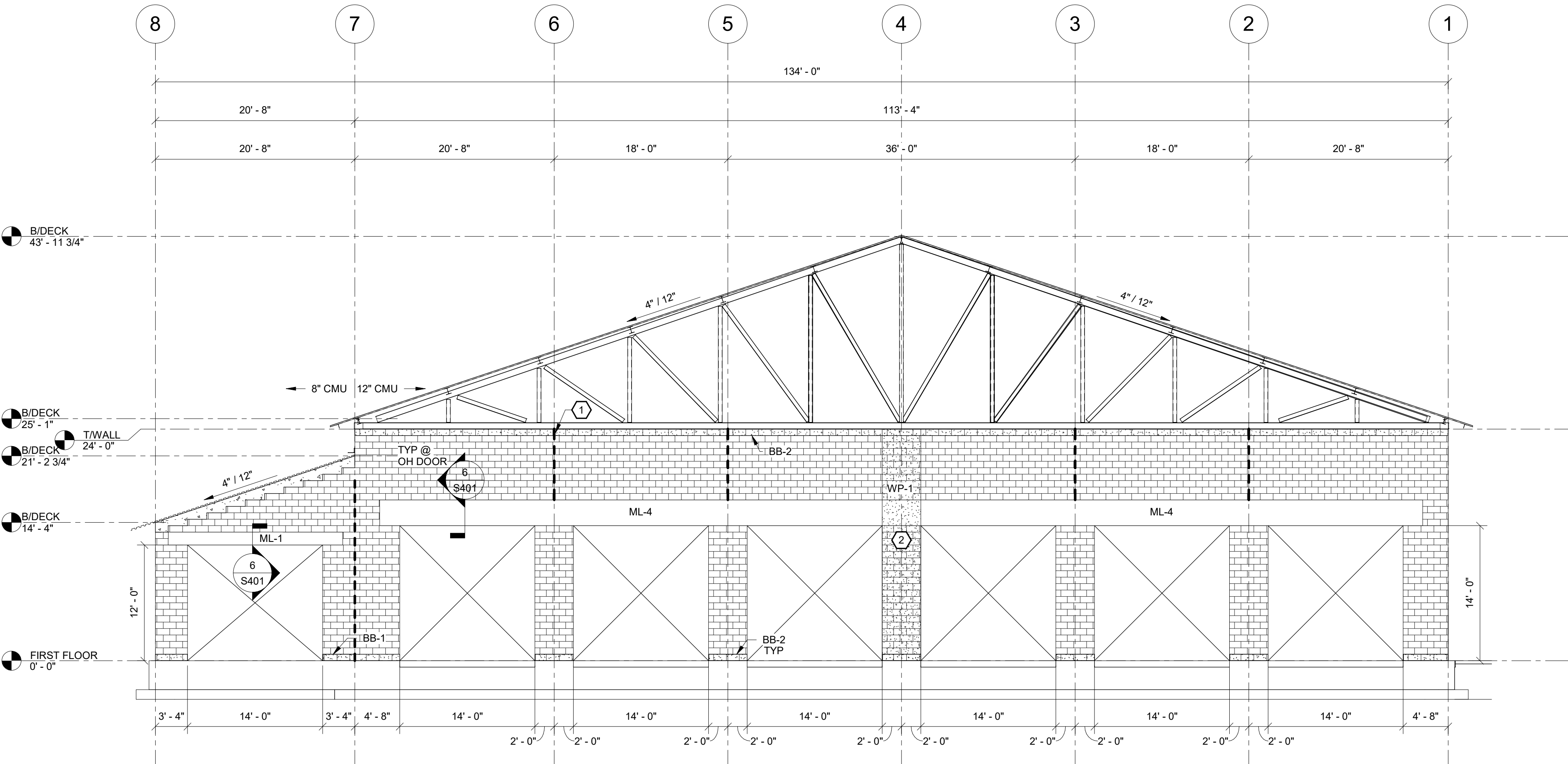
2 ELEVATION @ GRIDLINE E - ALTERNATE 1 1/8" = 1'-0"
