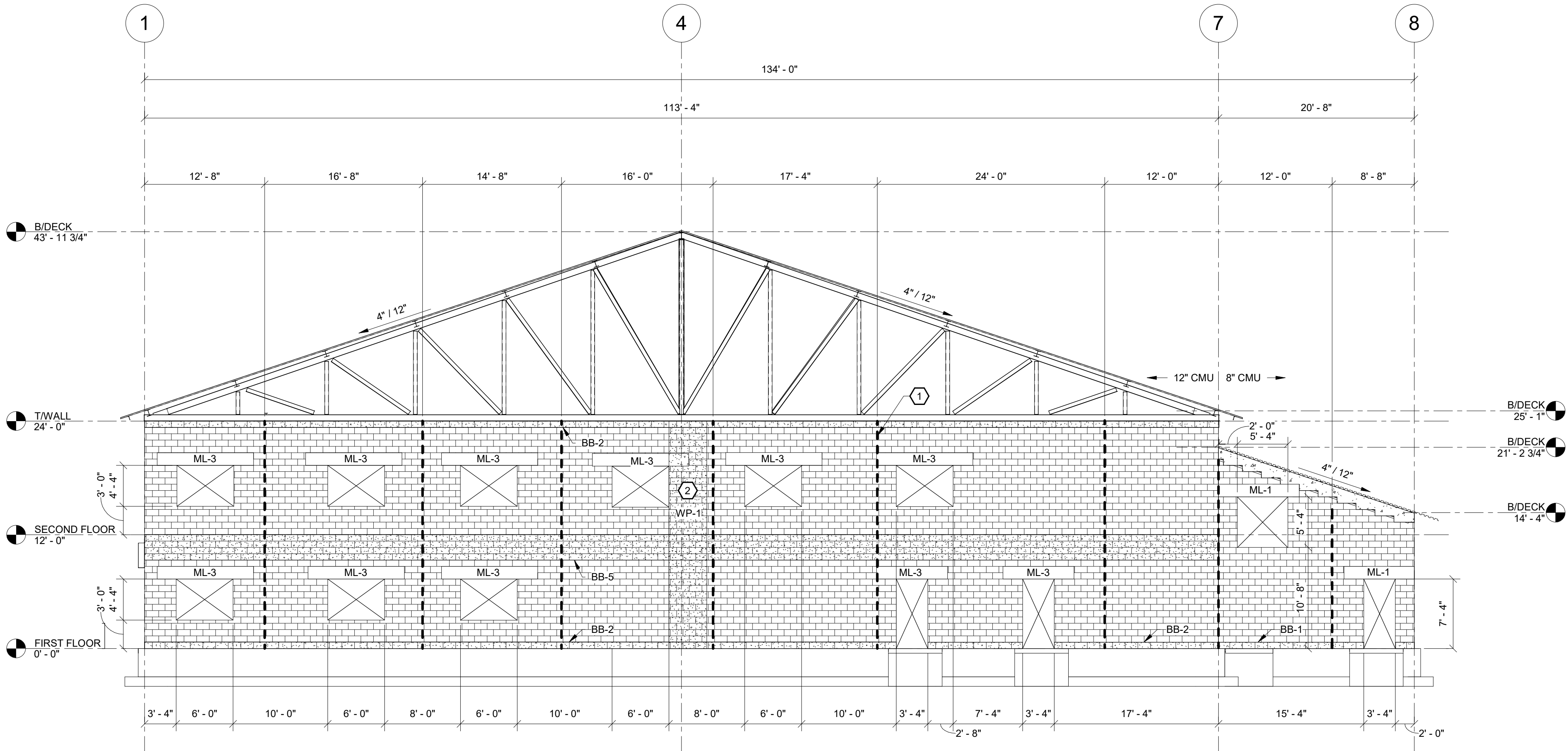
1 ELEVATION @ GRIDLINE A & C.1 - ALTERNATE 1 1/8" = 1'-0"
