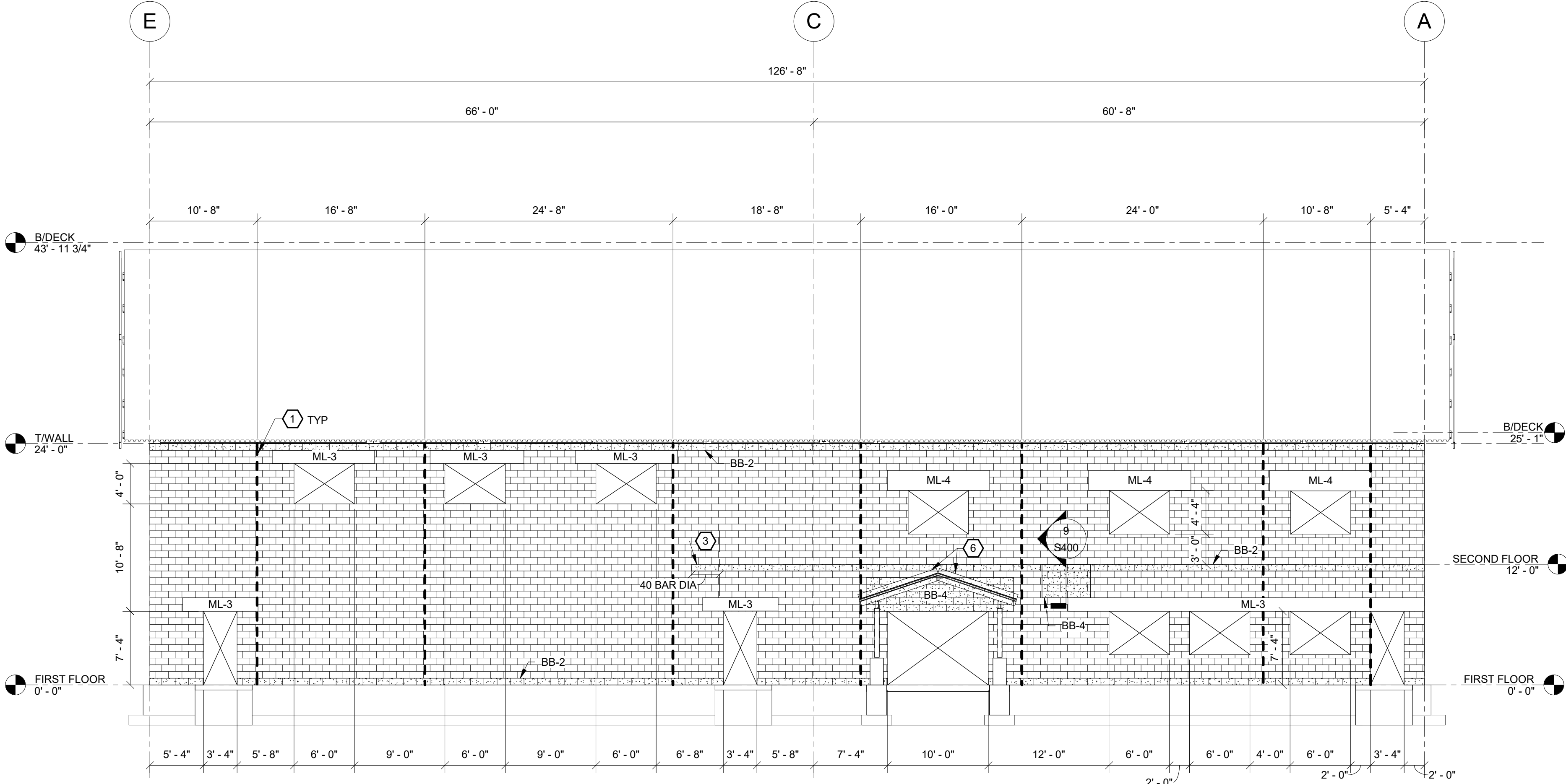
2 ELEVATION @ GRIDLINE 1 S201 1/8" = 1'-0"
