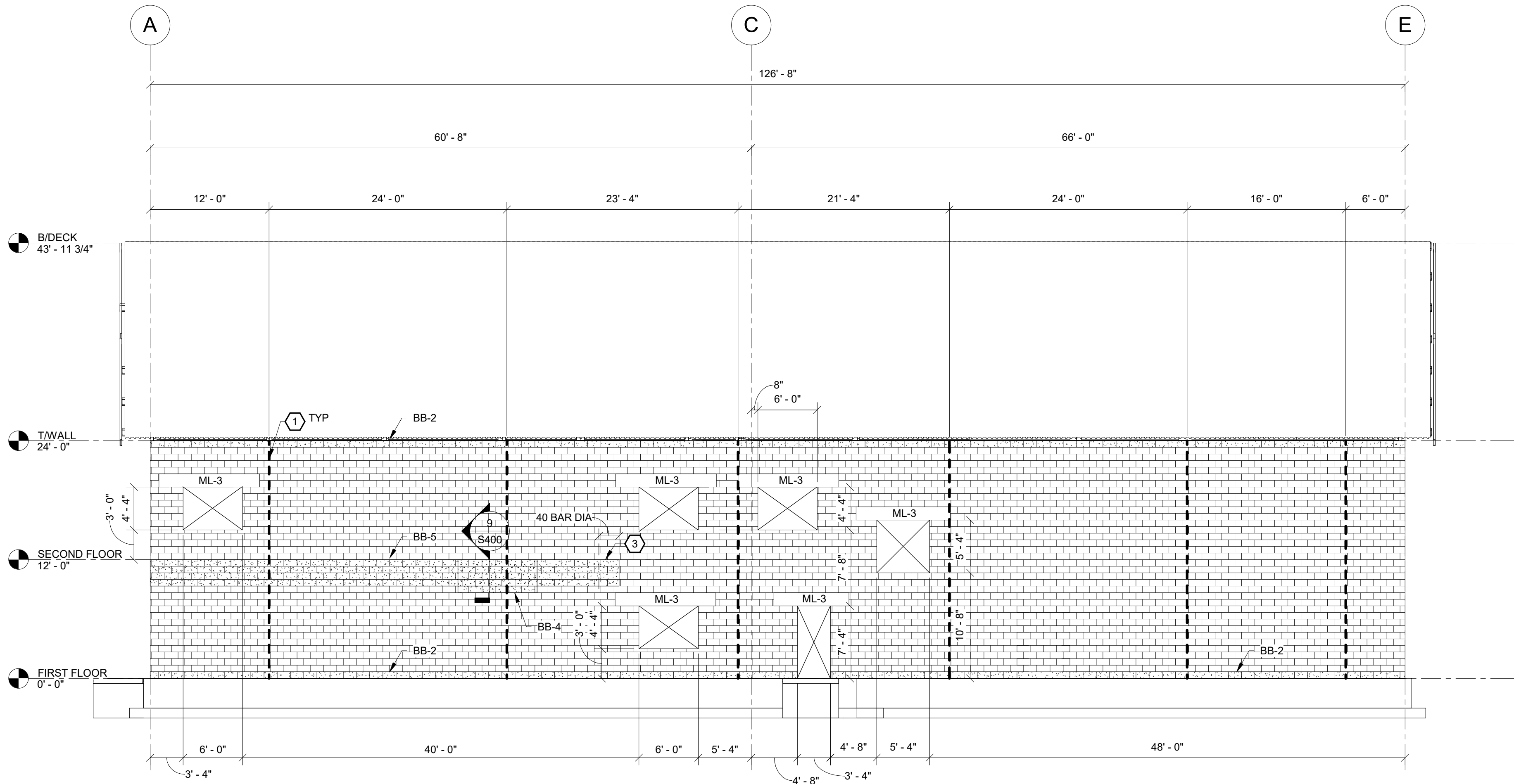
1 ELEVATION @ GRIDLINE 7 S201 1/8" = 1'-0"
