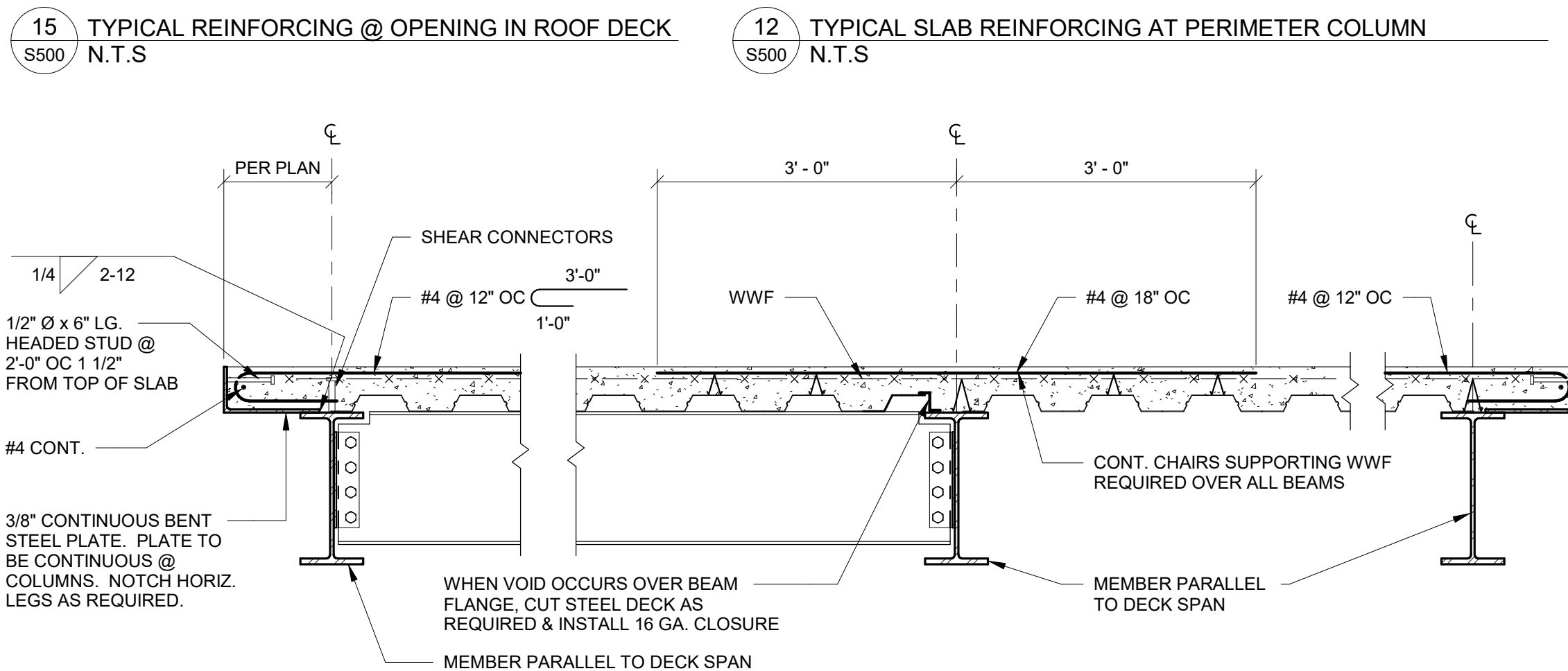
11 TYPICAL EDGE DETAIL & REINFORCING IN DECK SUPPORTED SLABS 500 N.T.S
