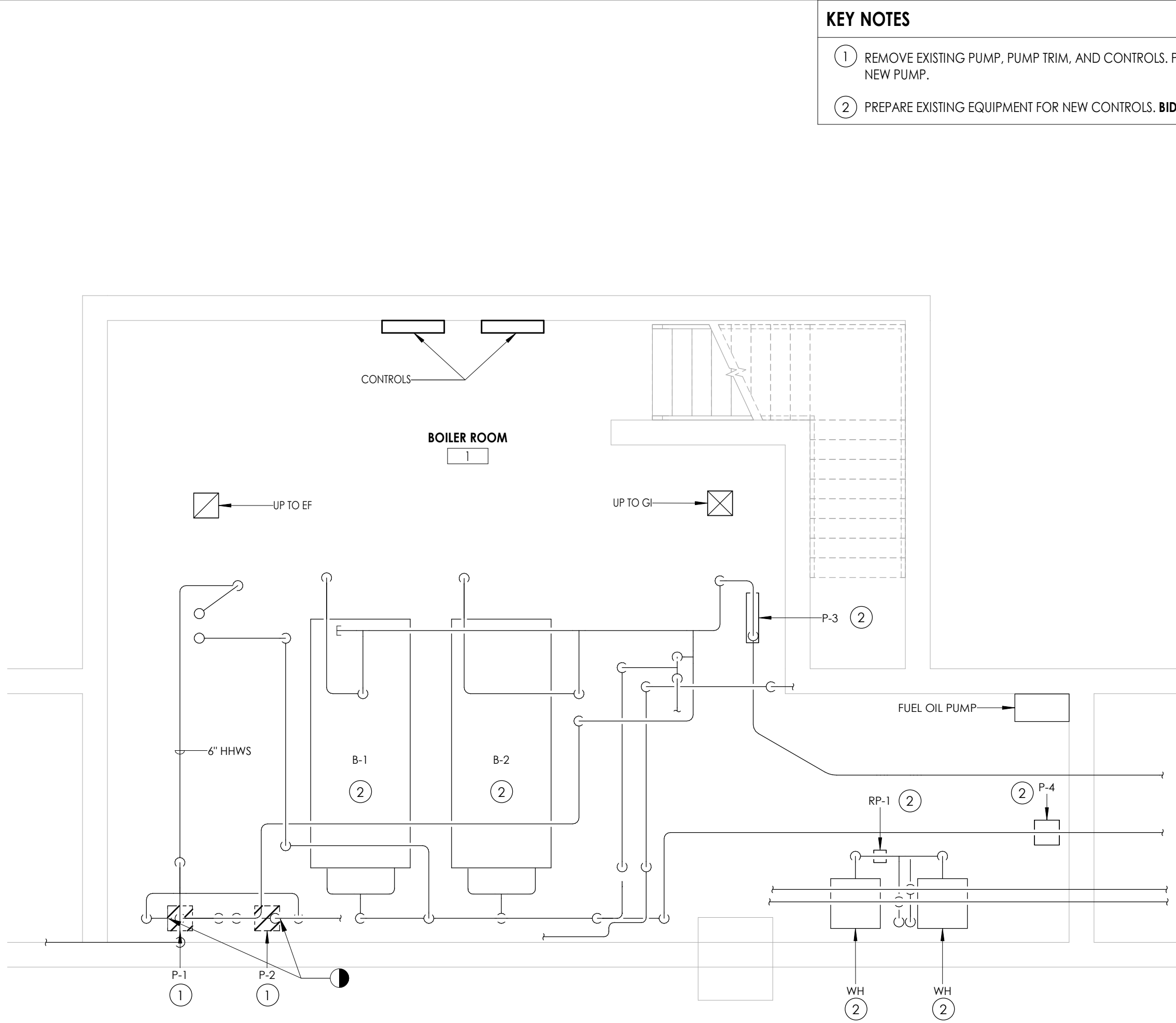
1 H100 BASEMENT BOILER ROOM DEMOLITION PLAN 1/4" = 1'-0"
