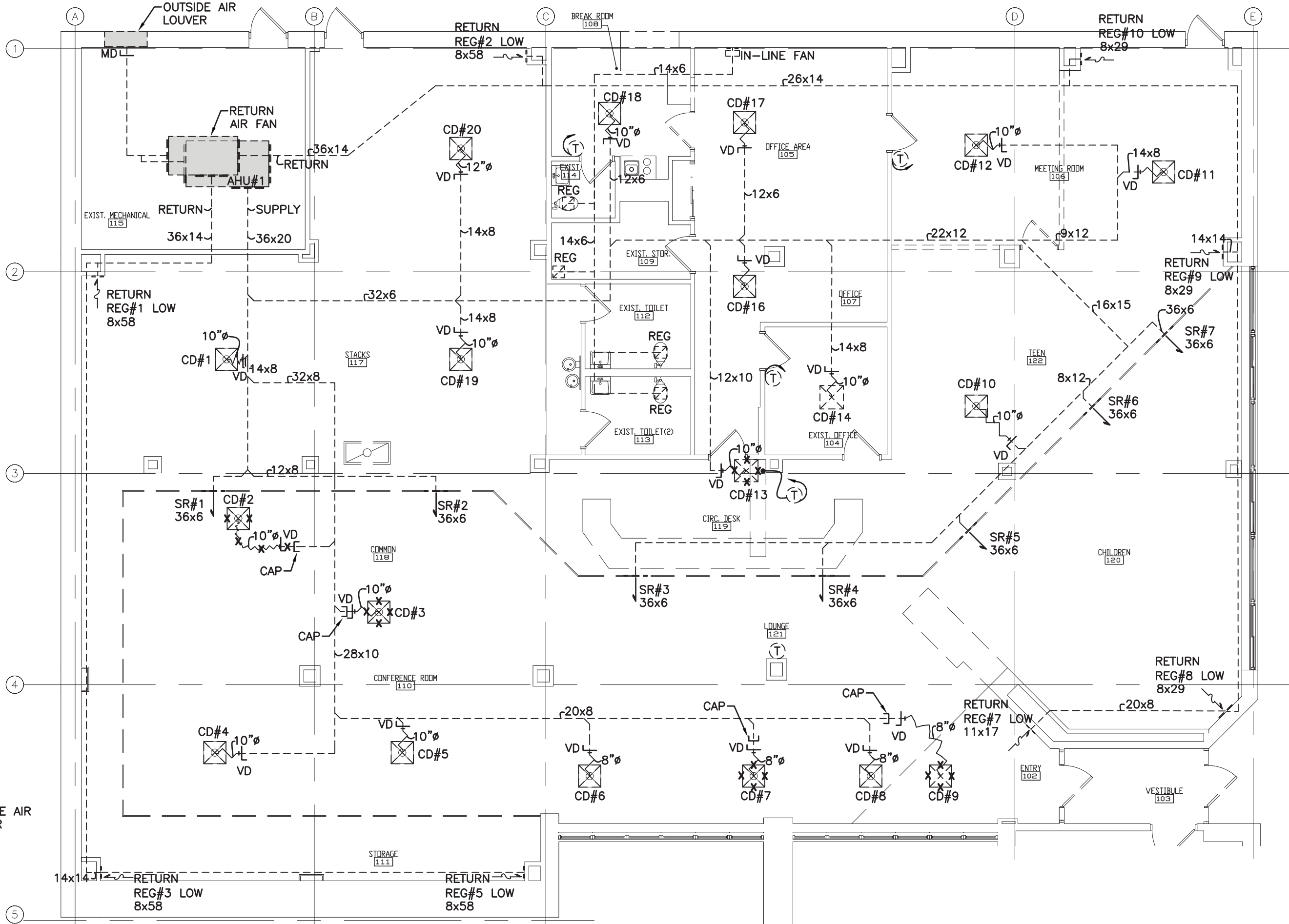
1 GROUND FLOOR PLAN - EXISTING/REMOVAL H-100 SCALE: 1/8" = 1'-0"
