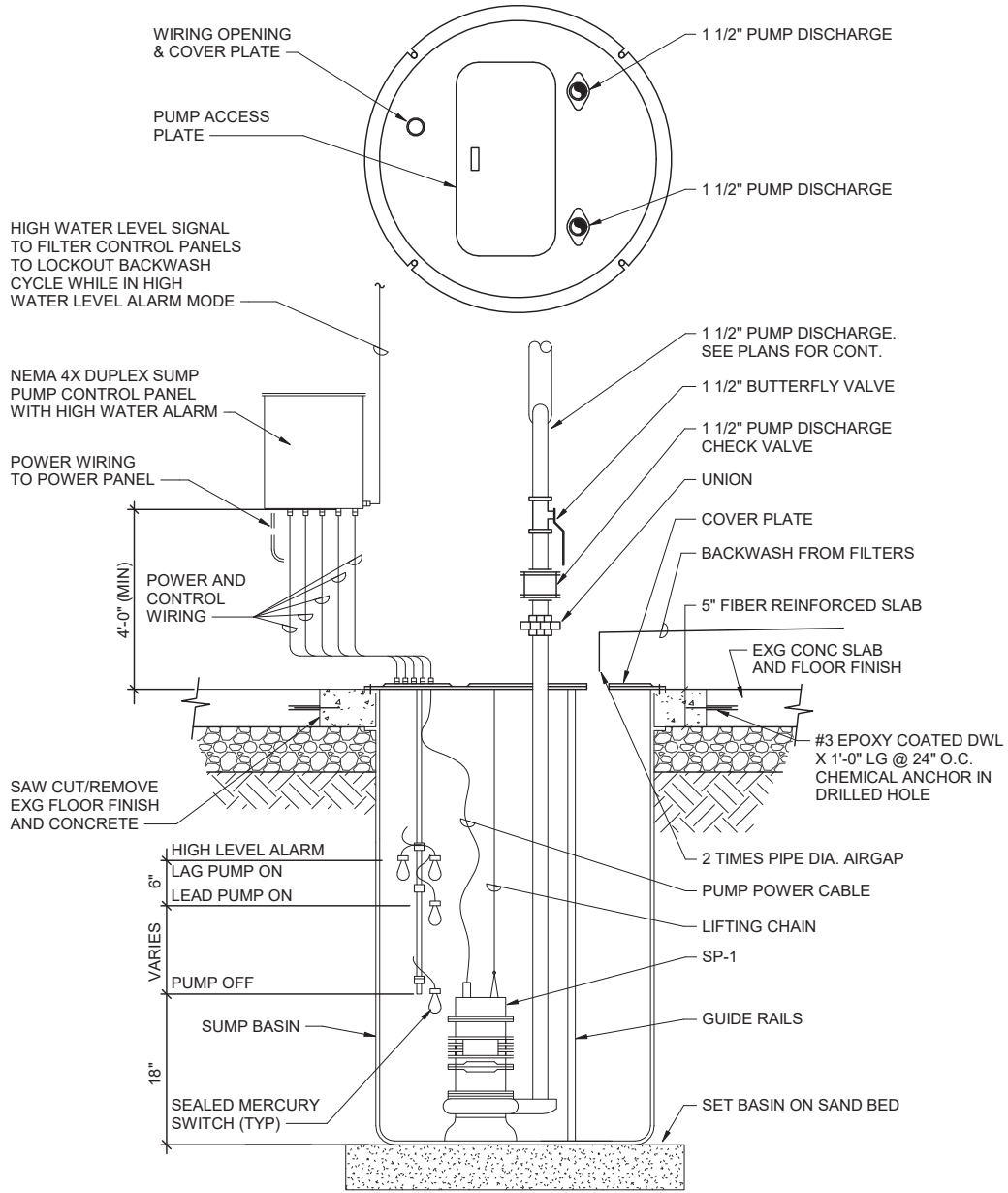
1 Duplex Sump Pump System Schematic NTS
