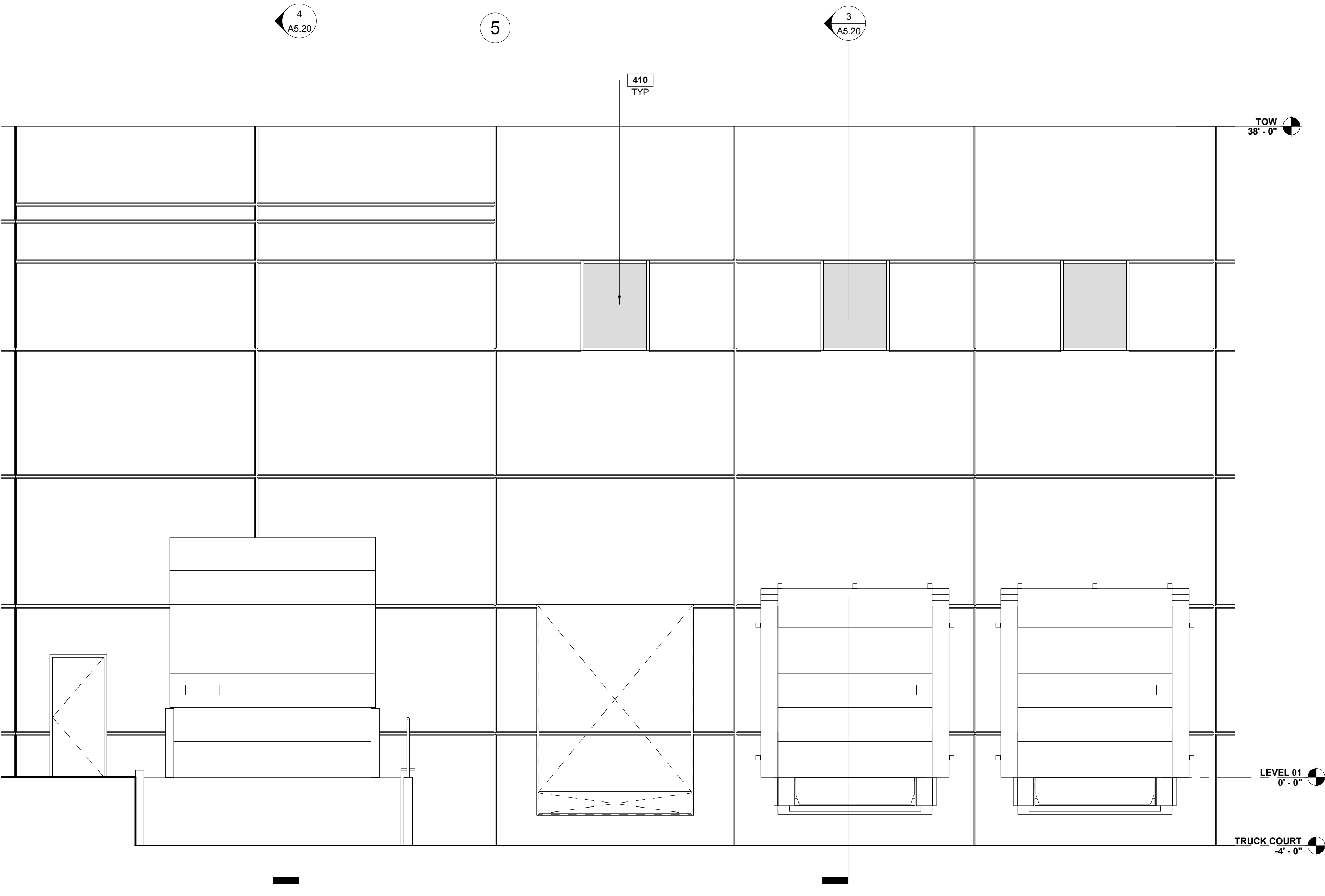
ENLARGED ELEVATION - DOCK WALL
