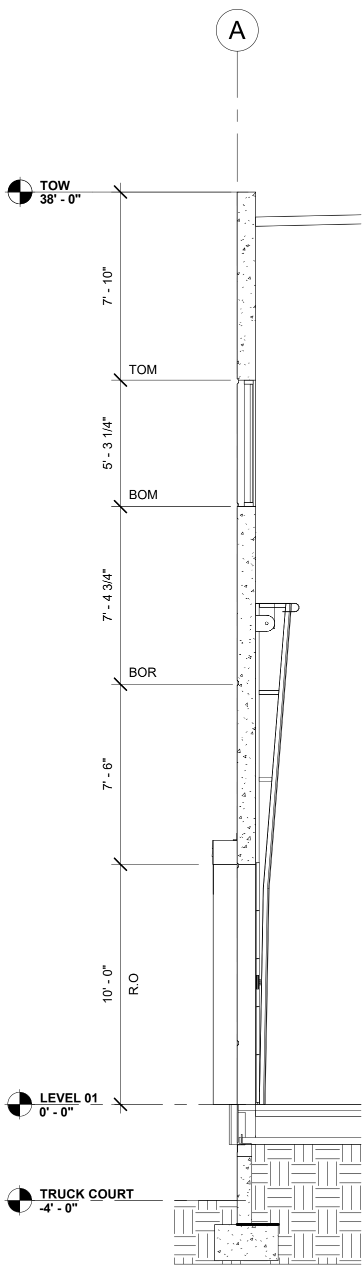
SECTION @ DOCK DOOR 3 SCALE: 1/4" = 1'-0"
