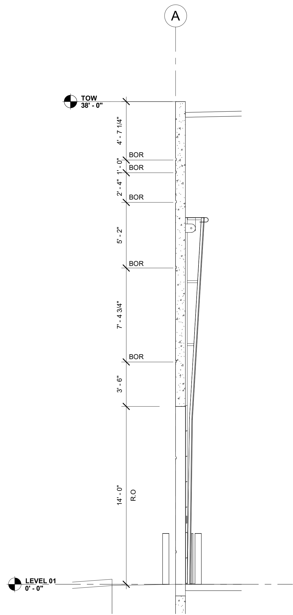
SECTION @ DRIVE-IN DOOR
