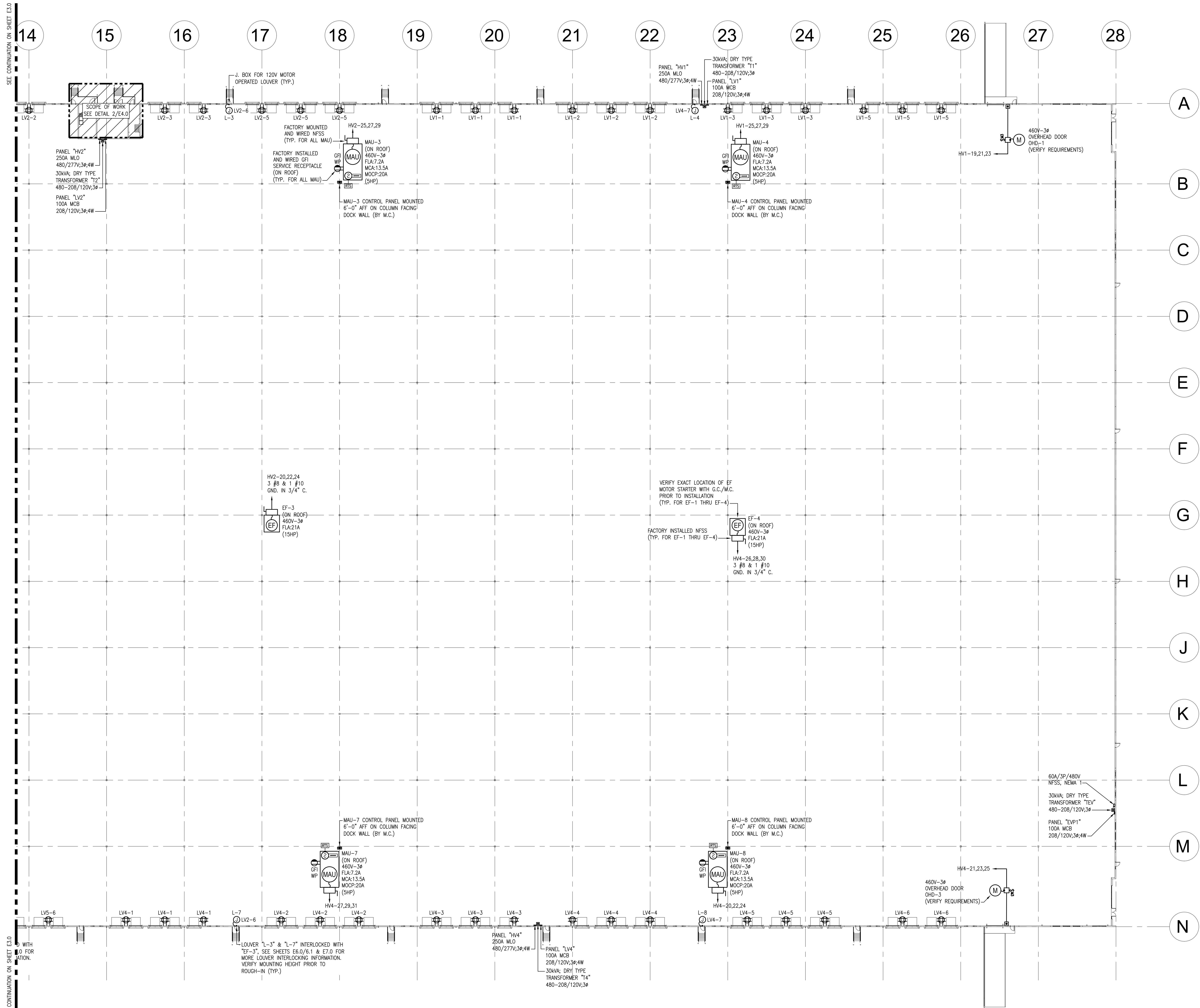
1 PARTIAL WAREHOUSE POWER PLAN E3.1 SCALE: 1" = 30'-0"
