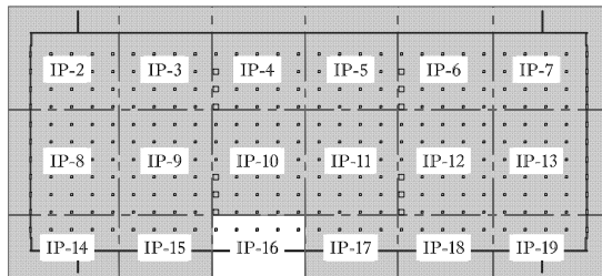
IMPACT PIER ELEMENT LAYOUT - PLAN VIEW - BUILDING 1
