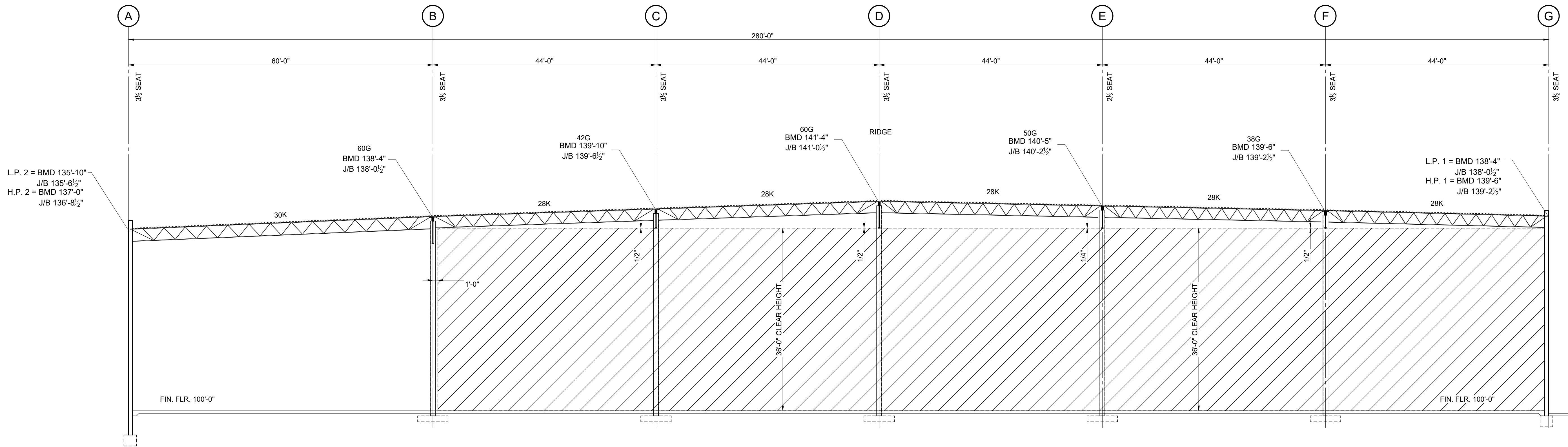
TYPICAL BUILDING CROSS-SECTION
