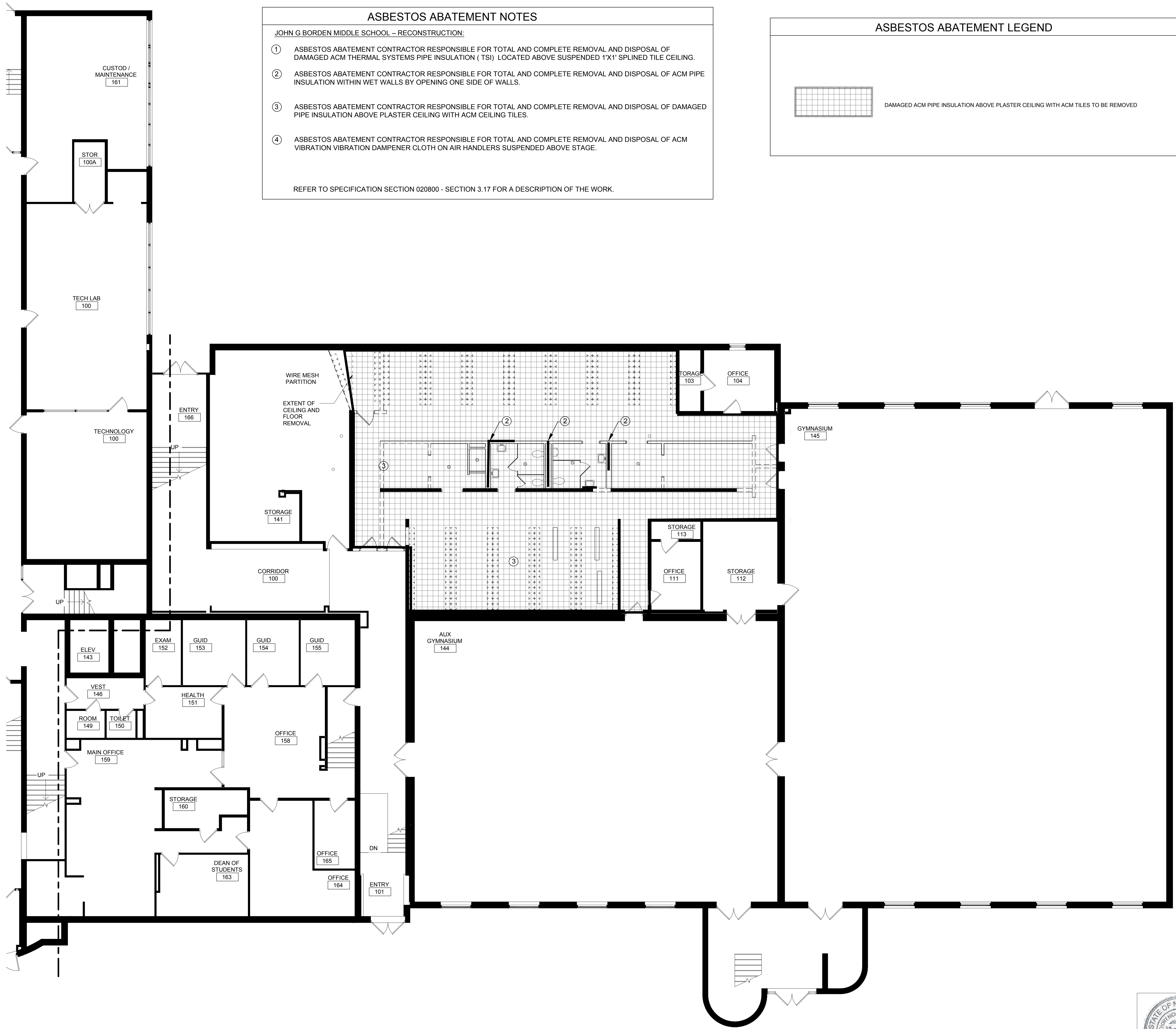
1 First Floor Abatement Plan- Area "B" 1/8" = 1'-0"
