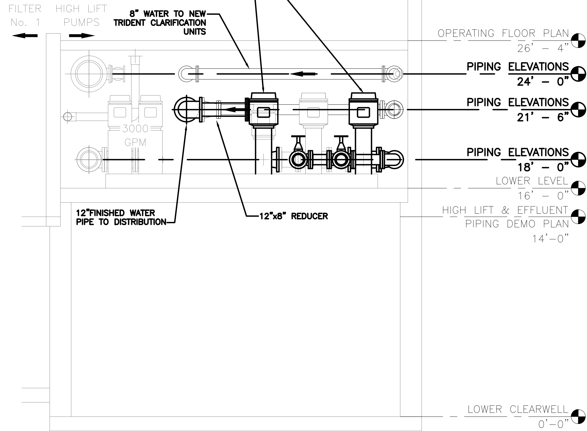
A HIGH LIFT PUMP NEW PIPING SECTION C-202 SCALE: 1/4"=1'-0"
