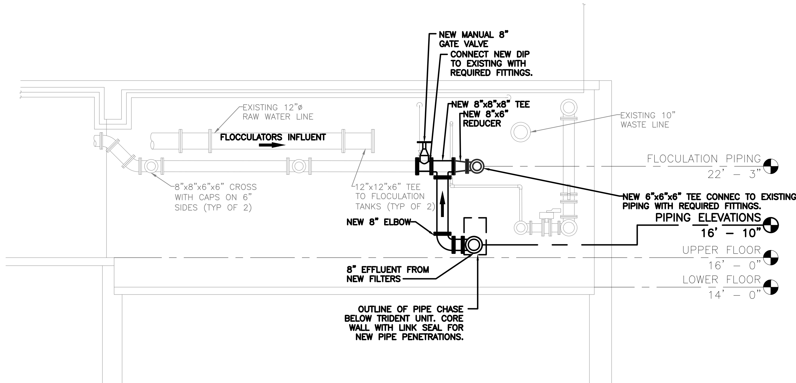
D TRIDENT NEW PIPING SECTION C-203 SCALE: 1/4"=1'-0"
