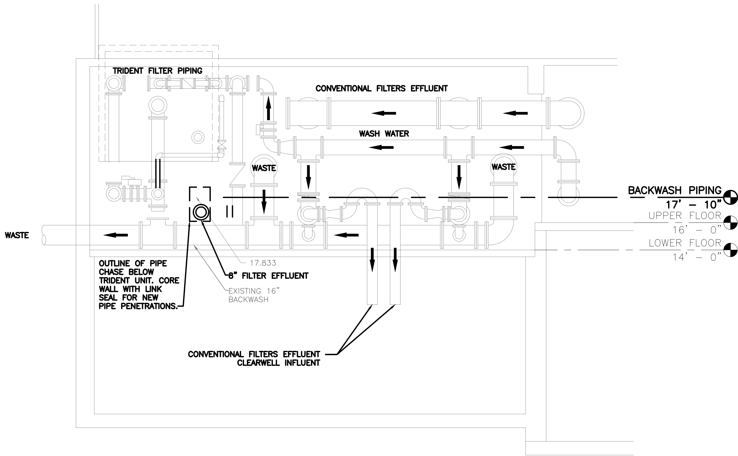
C TRIDENT NEW PIPING SECTION C-203 SCALE: 1/4"=1'-0"
