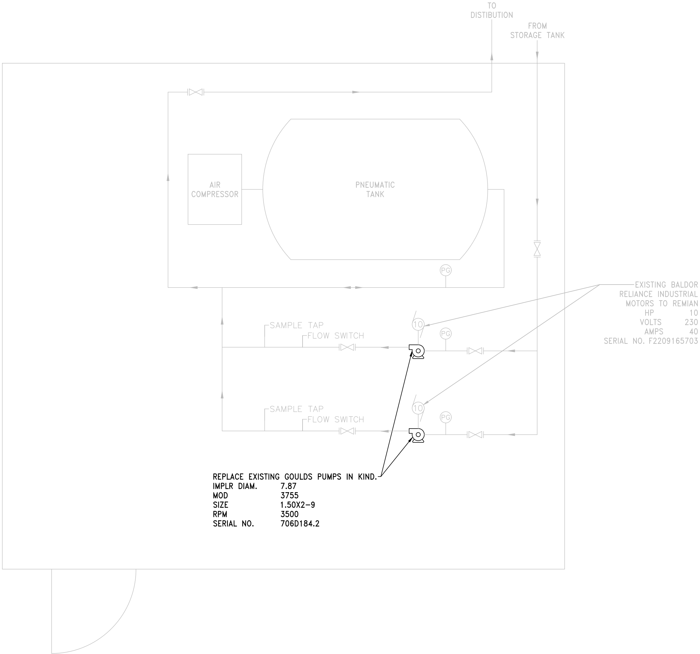
VIOLET HILL PUMP STATION FLOOR PLAN SCHEMATIC NOT TO SCALE
