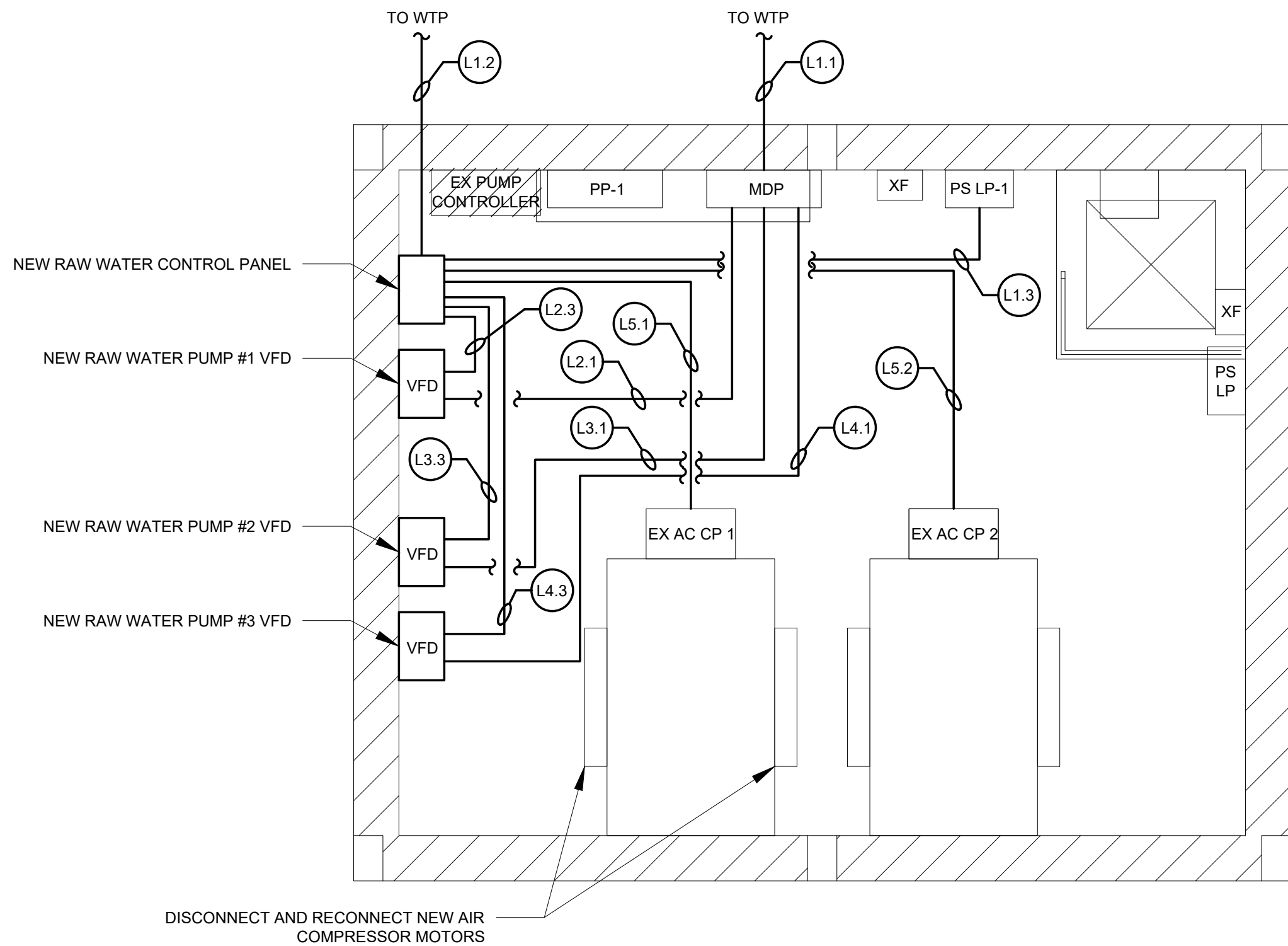
RAW WATER PUMP STATION UPPER LEVEL ELECTRICAL PLAN SCALE: 3/8" = 1'
