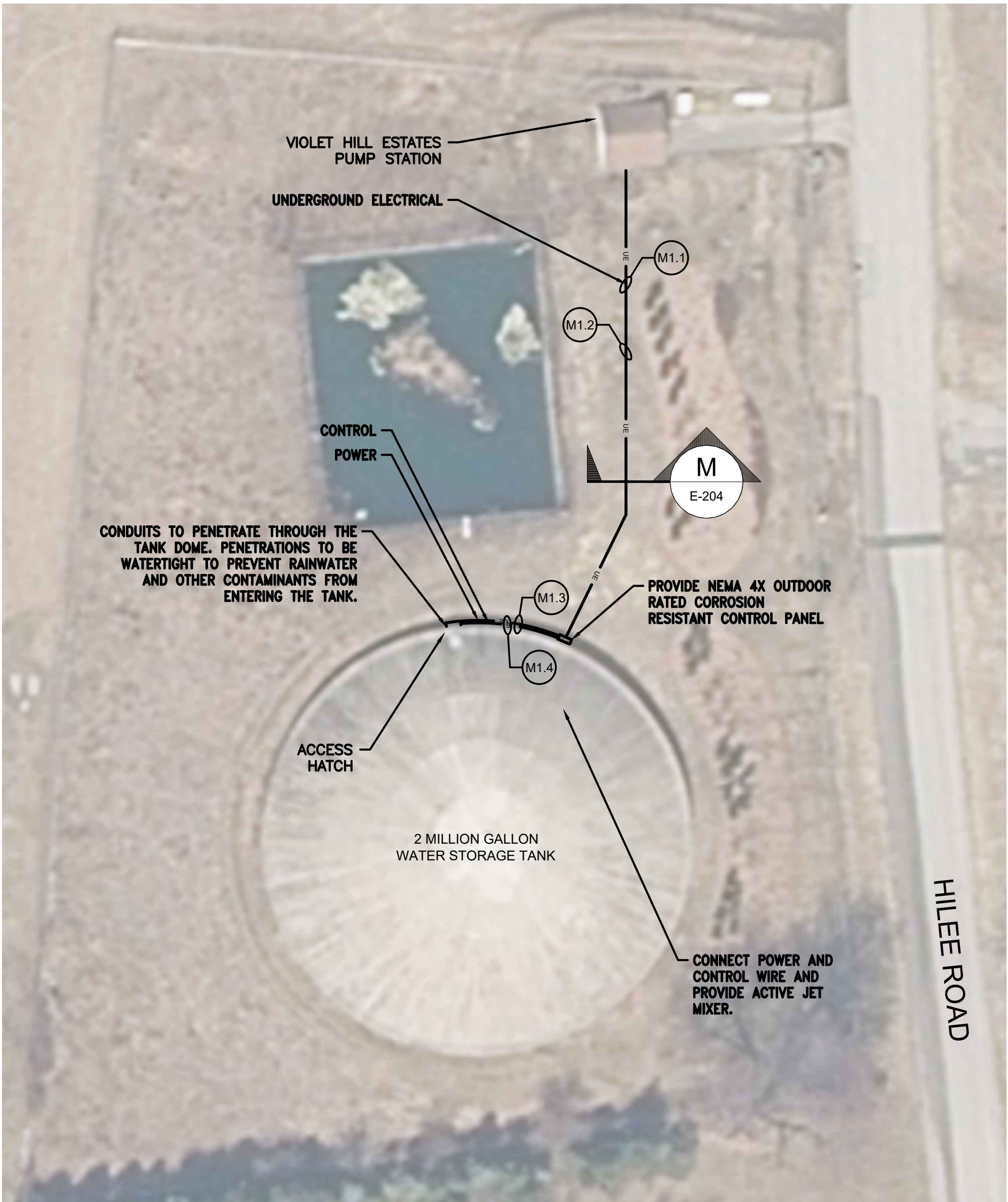
MIXER ELECTRICAL PLAN SCALE: 1" = 30'
