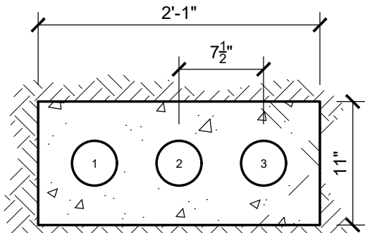
DUCT BANK SECTION A, B, C
