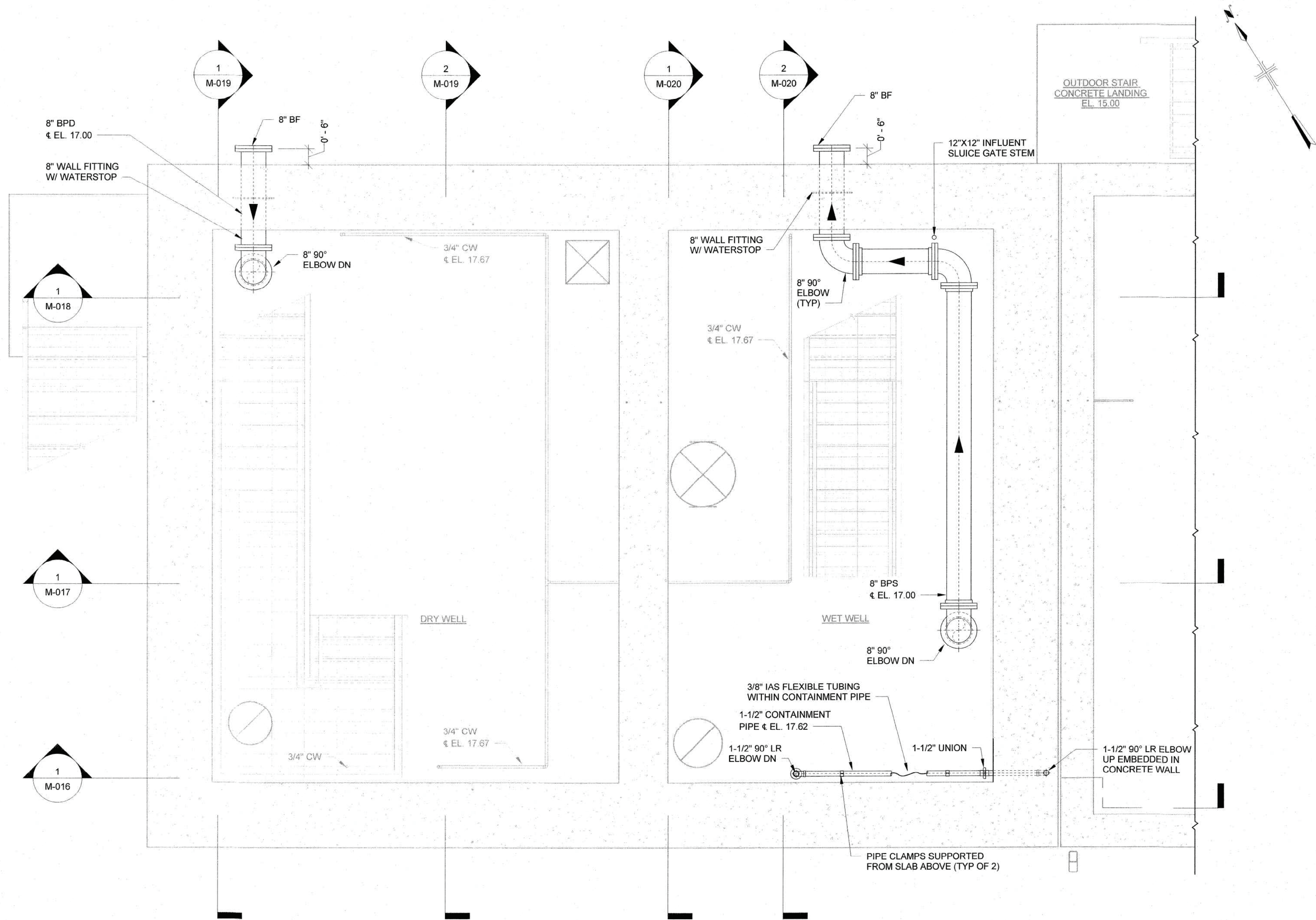
UPPER LEVEL - PARTIAL PLAN AT EL. 14.20
