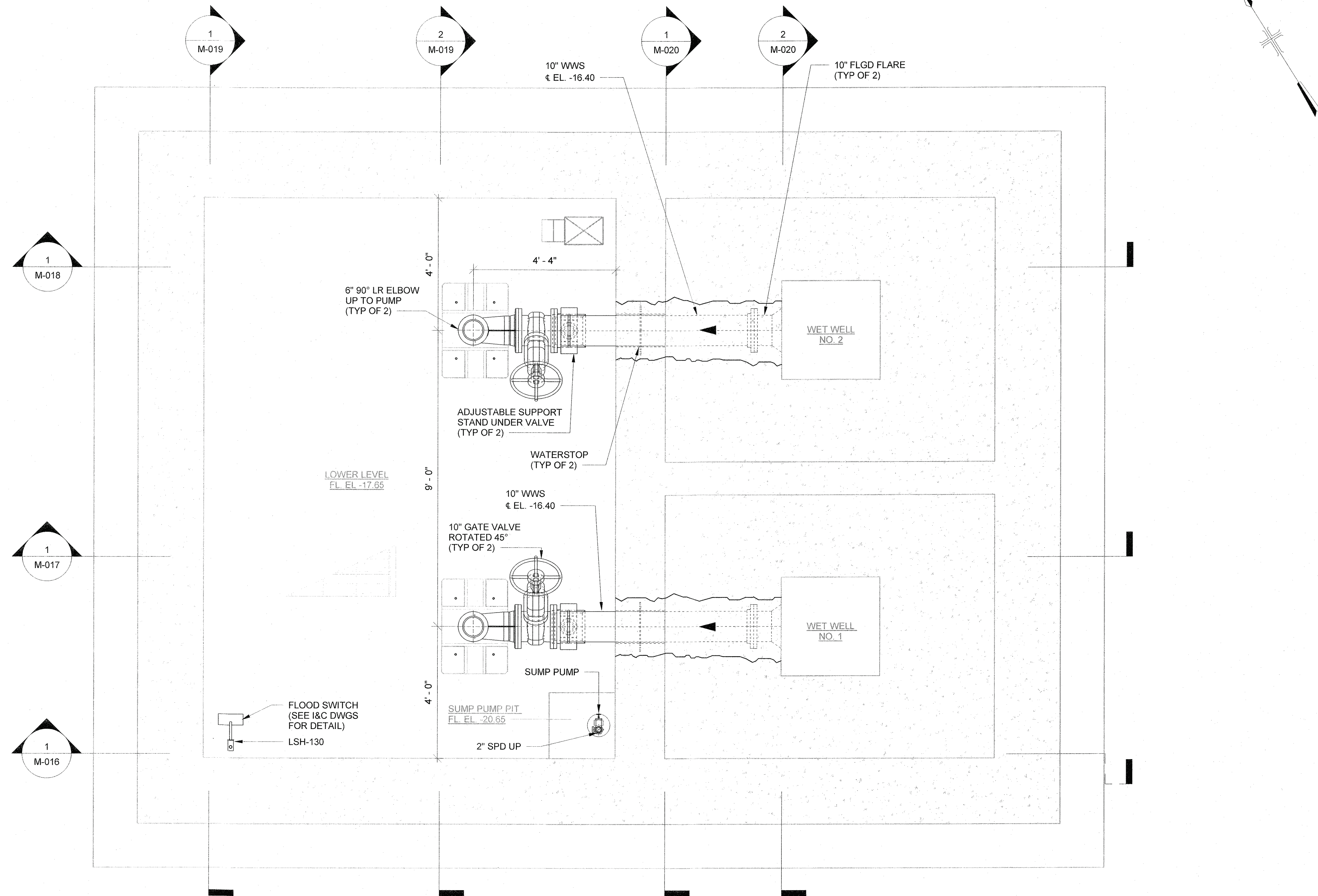
LOWER LEVEL - PLAN AT EL. -17.65
