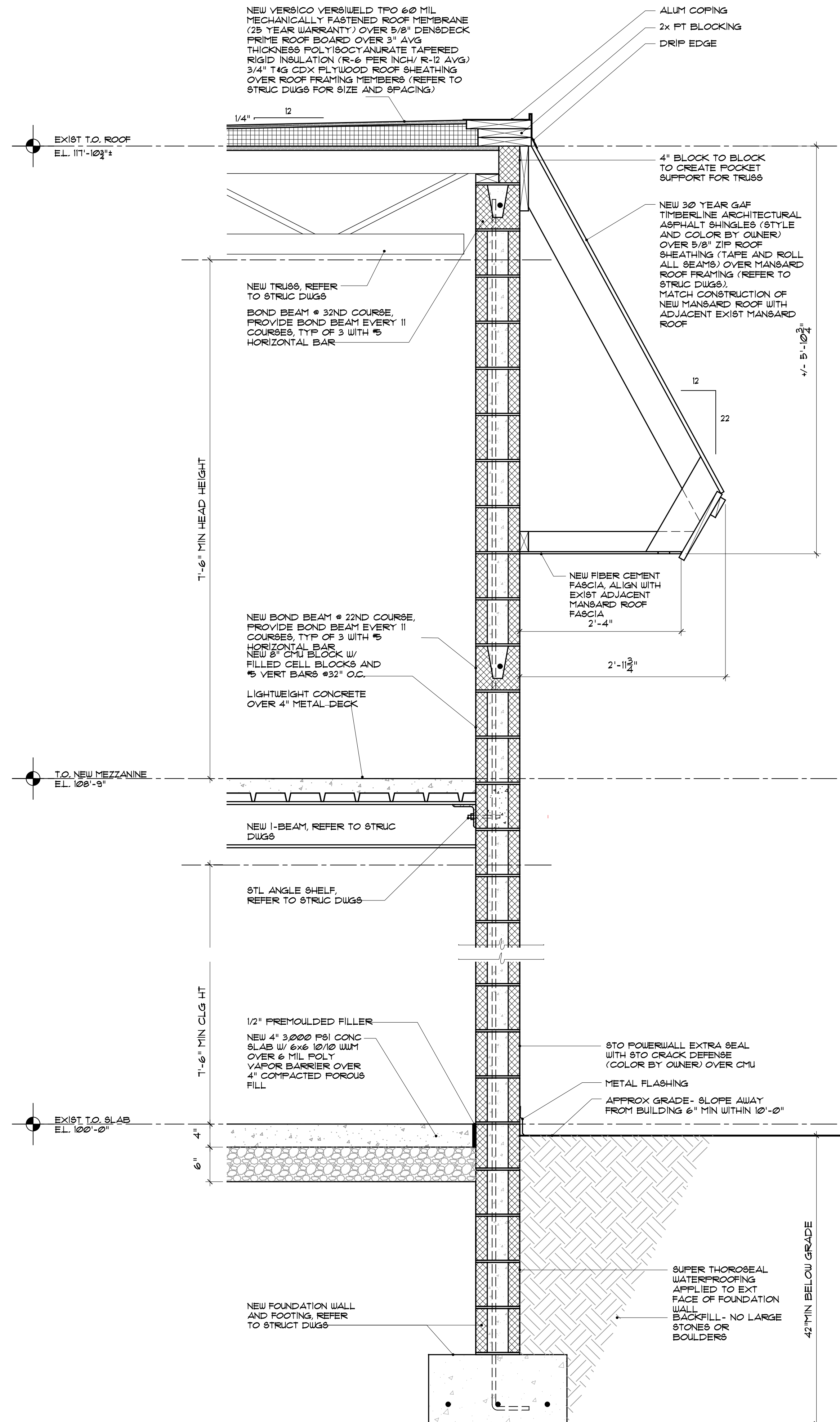
1 Wall Section at New Storage Addition A3.03 Scale: 1" = 1'-0"
