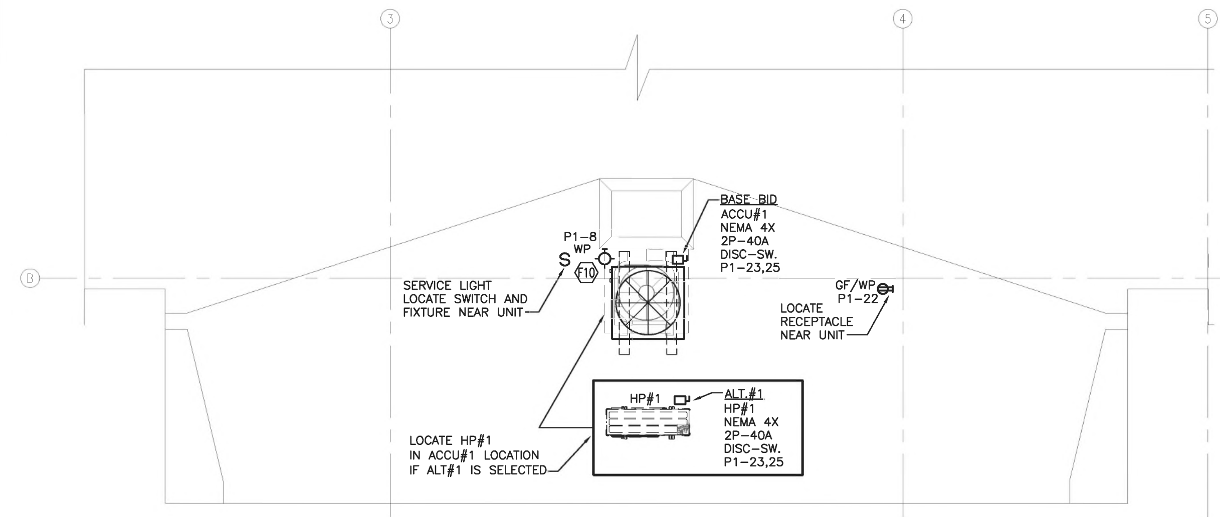
3 PARTIAL ROOF PLAN - POWER/LIGHTING E-100 SCALE: 1/4" = 1'-0" NORTH
