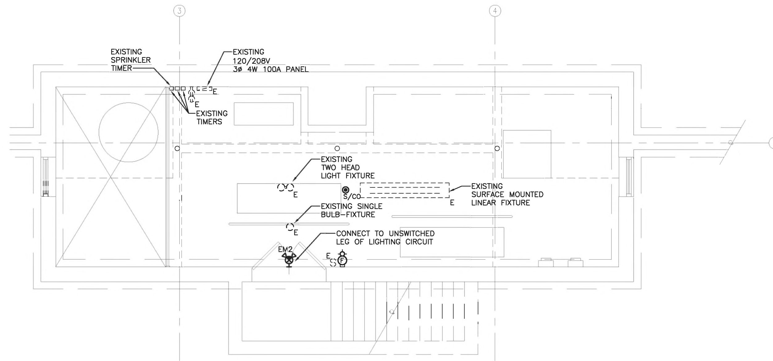
2 PARTIAL CELLAR PLAN - POWER/LIGHTING E-100 SCALE: 1/4" = 1'-0" NORTH
