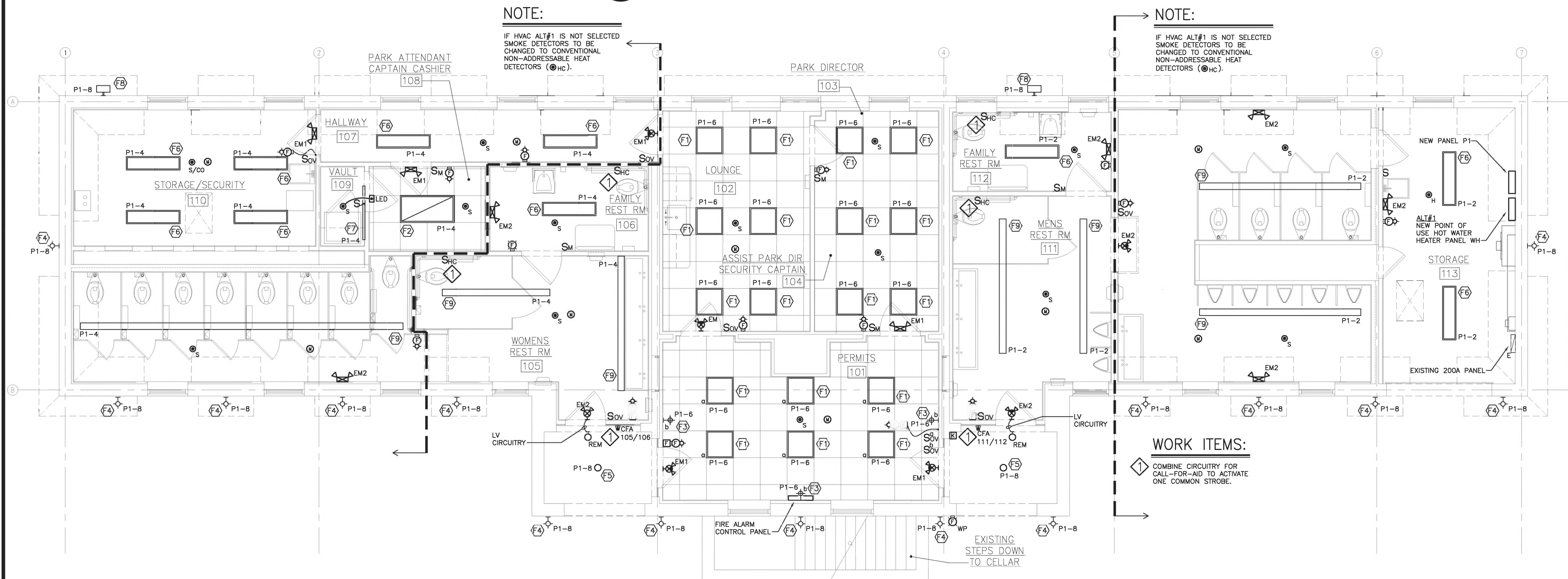
1 E-101 PROPOSED FLOOR PLAN - LIGHTING SCALE: 1/4" = 1'-0"
