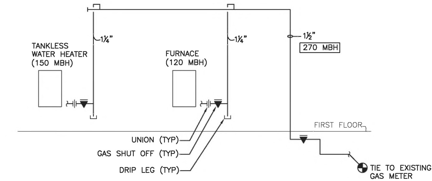
3 GAS RISER DIAGRAM P-101 NOT TO SCALE
