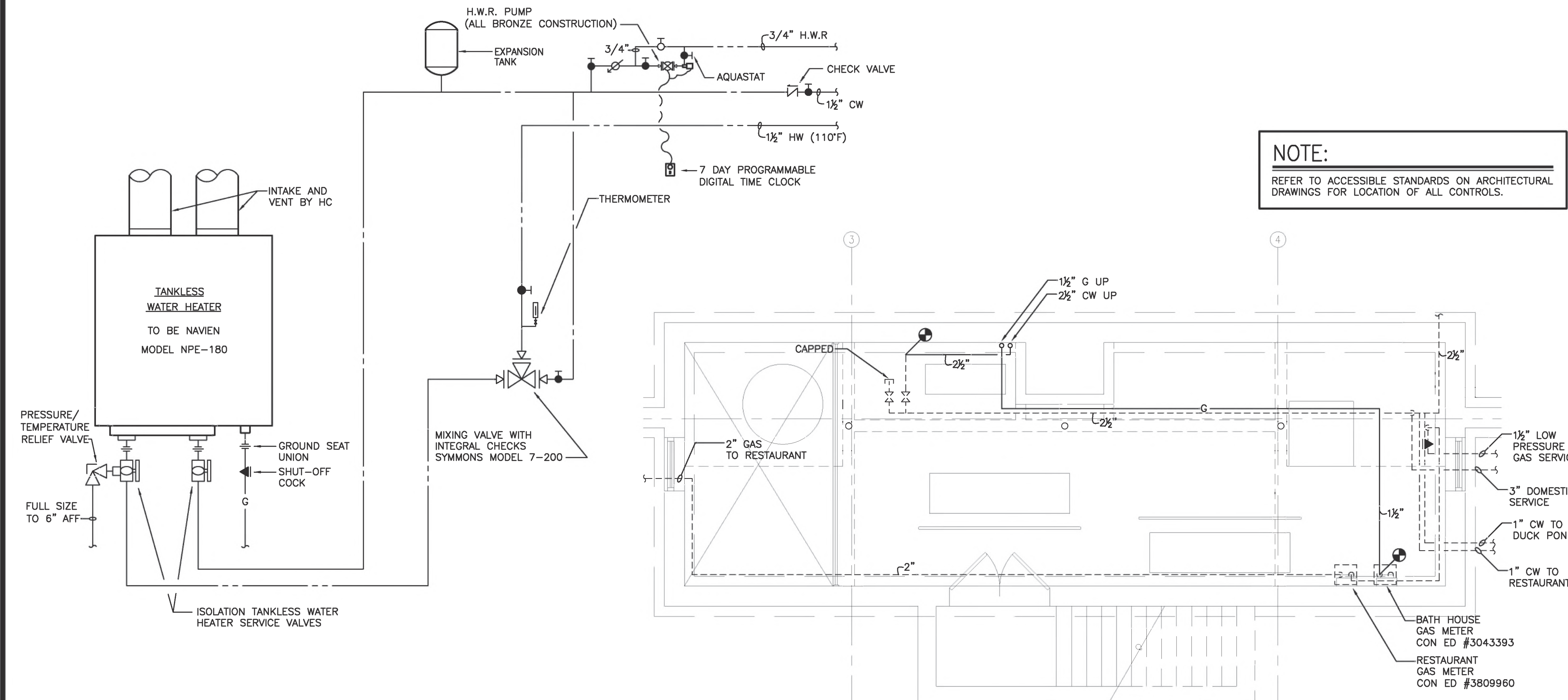
3 TANKLESS WATER HEATER PIPING P-100 NOT TO SCALE
