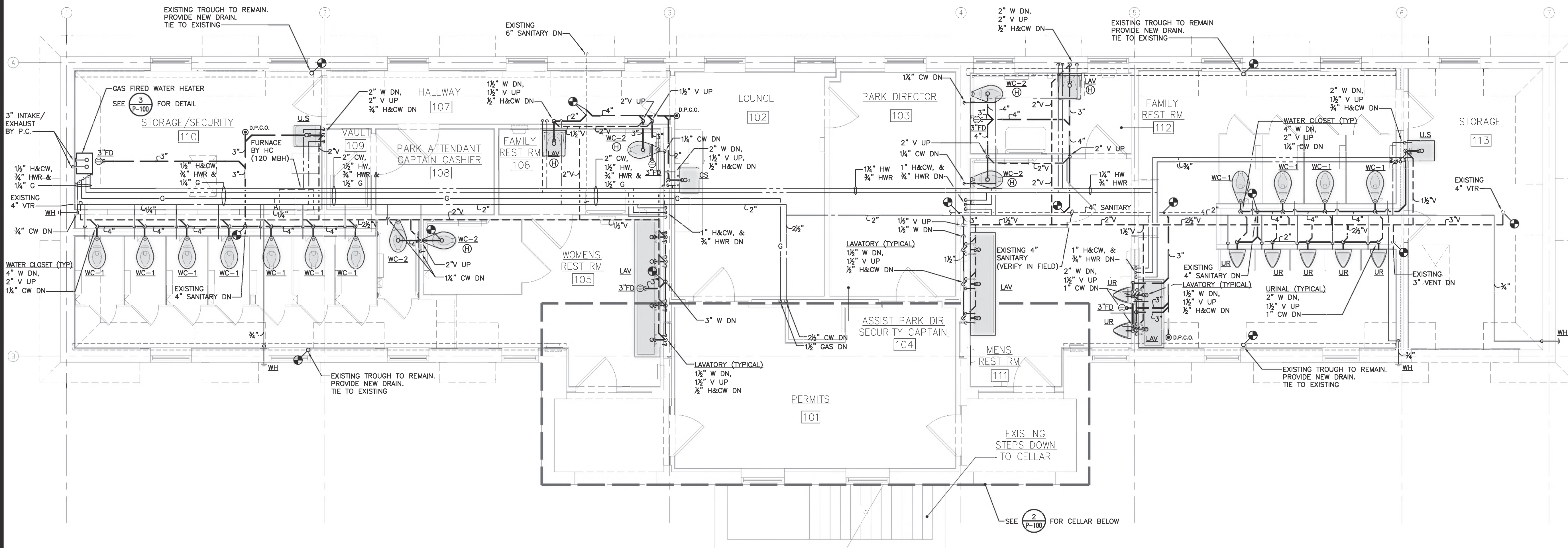
1 PROPOSED FLOOR PLAN - PLUMBING P-100 SCALE: 1/4" = 1'-0"
