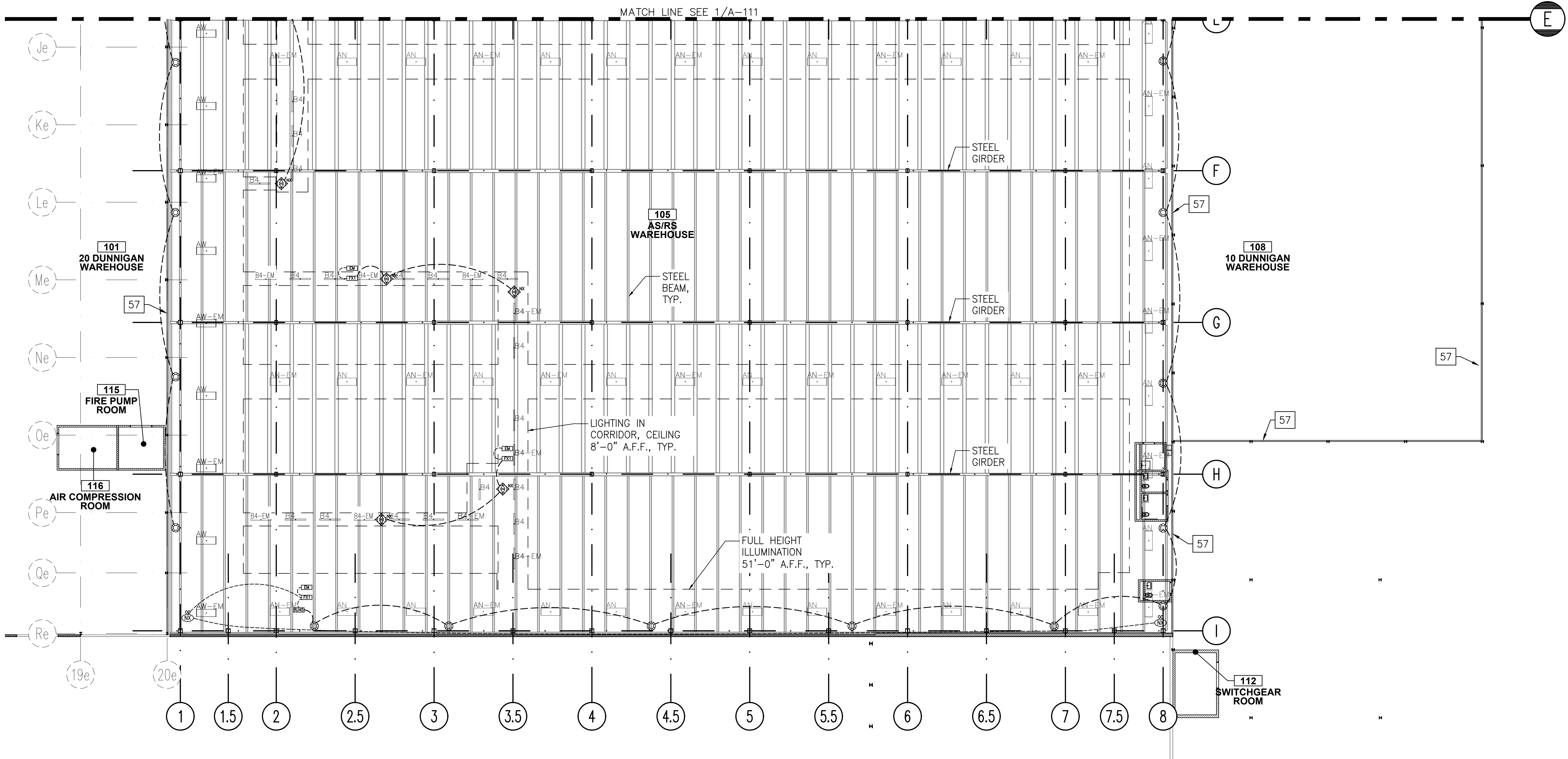
1 PROPOSED RCP - AS/RS WAREHOUSE (SOUTH) A-112 A-112 SCALE: 1/16"=1'-0"
