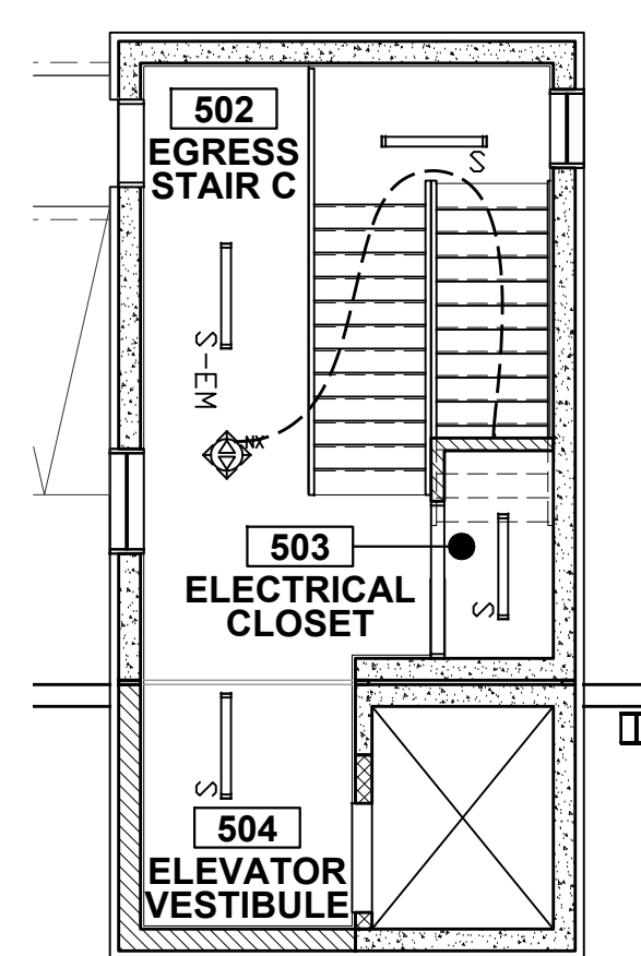
STAIR C ROOF RCP SCALE: 1/8"=1'-0"
