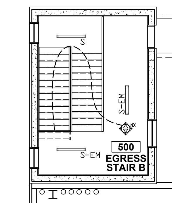
STAIR B ROOF RCP SCALE: 1/8"=1'-0"
