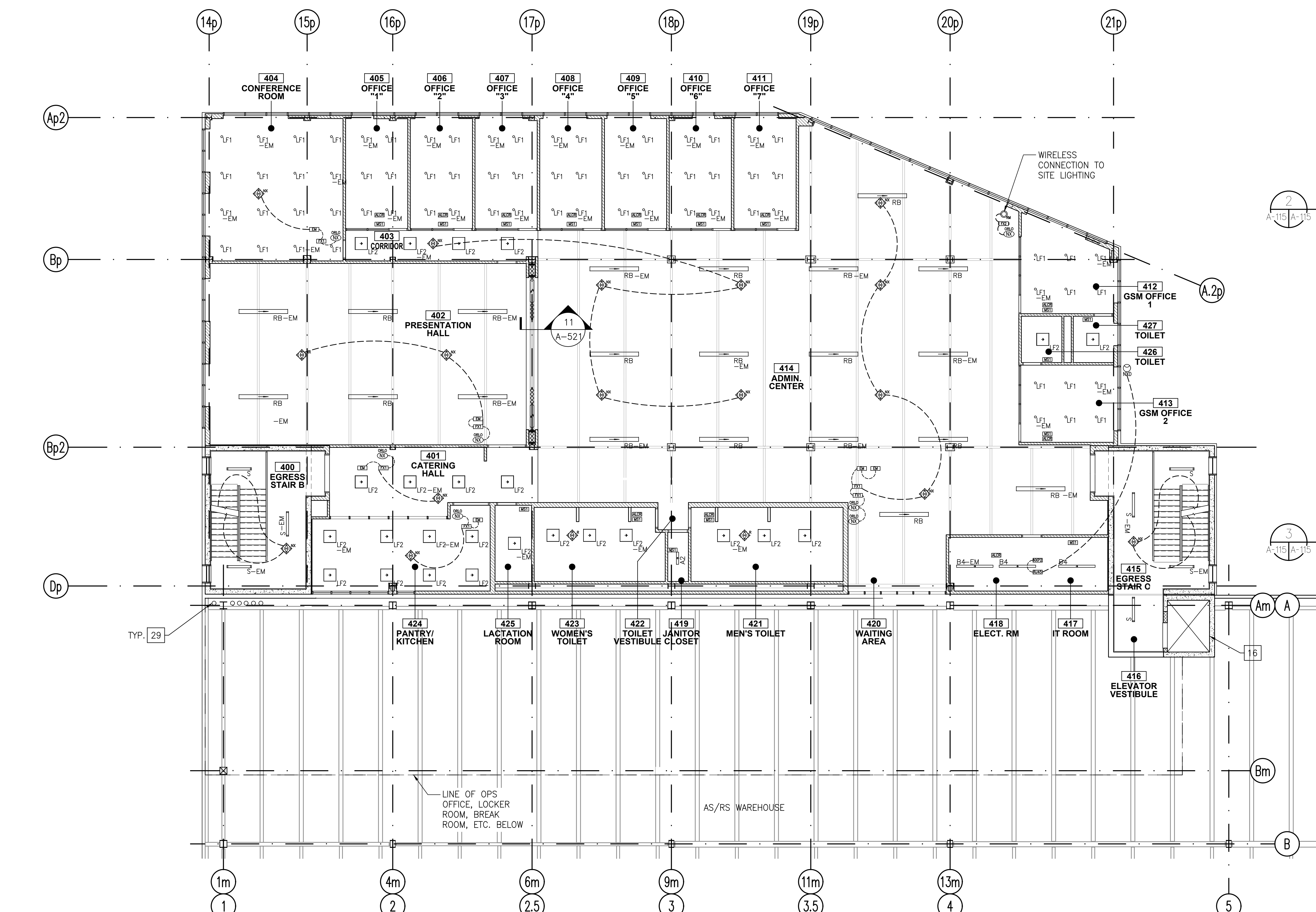
1 ENLARGED RCP - ADMIN. OFFICE SCALE: 1/8"=1'-0"
