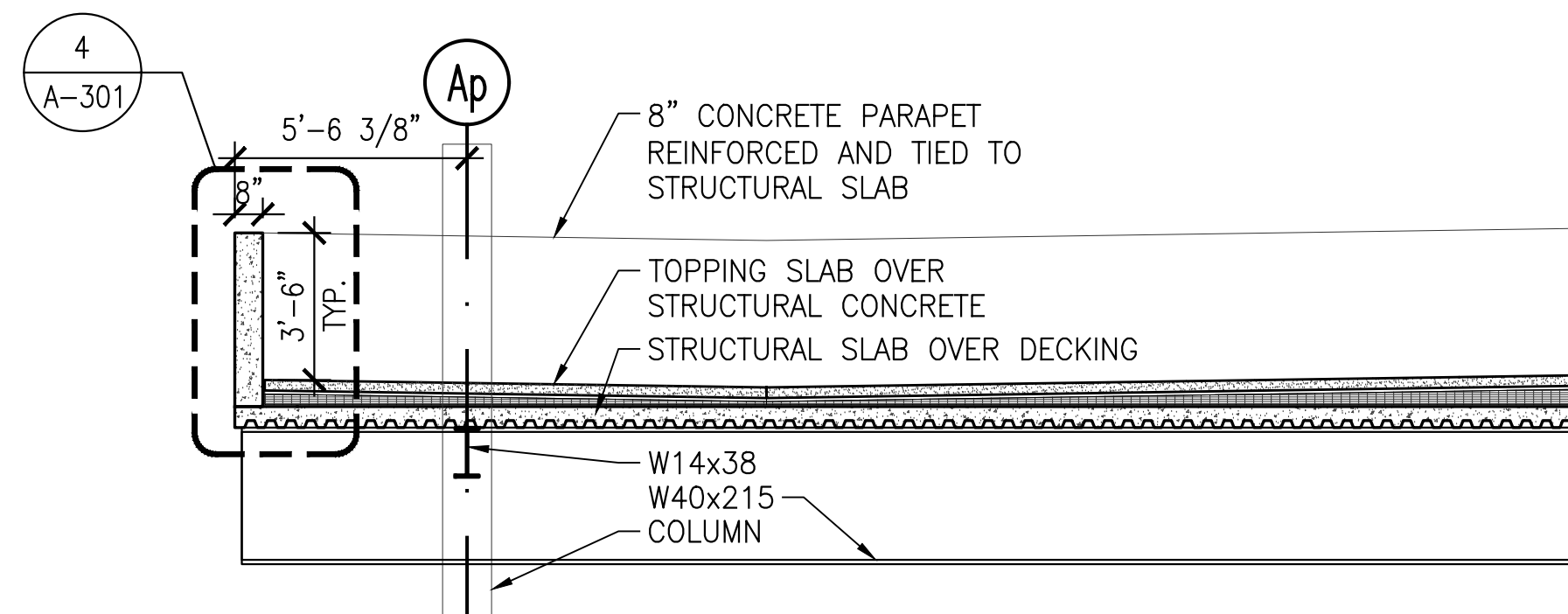
2 ENLARGED SECTION - END OF PARKING DECK A-210 A-210 SCALE: 1/4"=1'-0"
