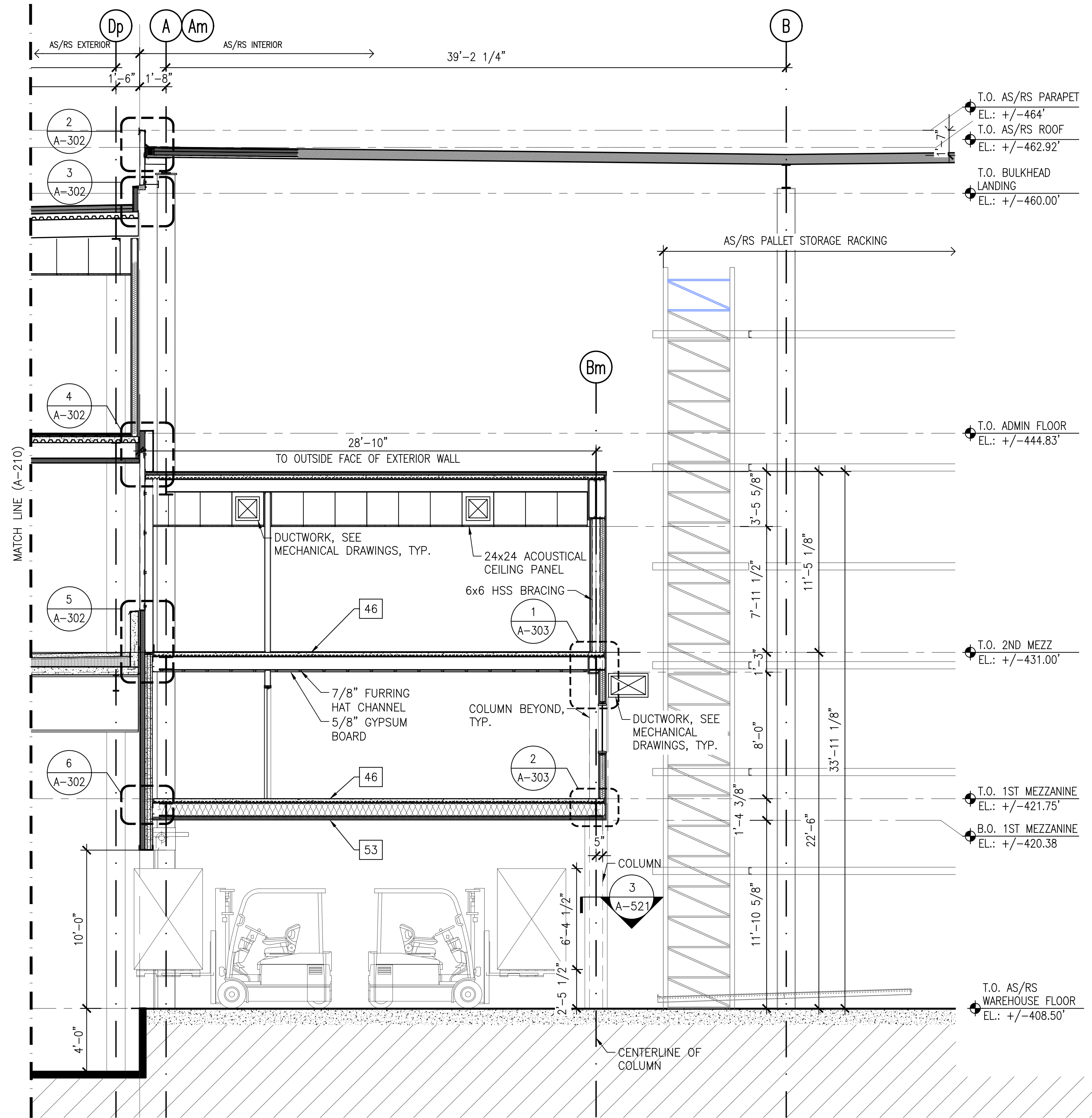
1 A-200 A-211 ENLARGED SECTION - OPERATION'S OFFICE AND AS/RS WAREHOUSE SCALE: 1/4" = 1'-0" 0 2 4 8 FT
