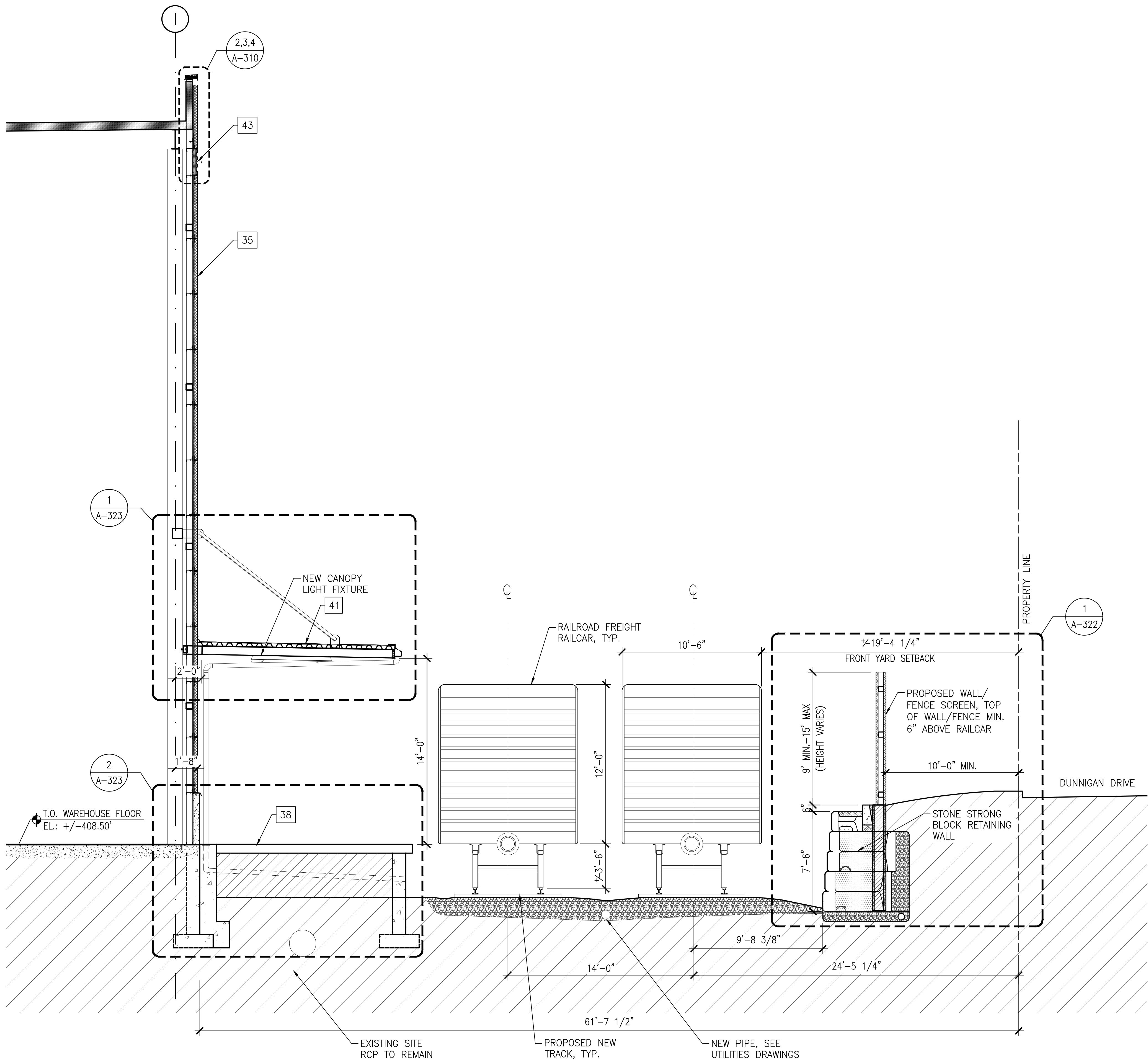
1 ENLARGED SECTION - SOUTH PLATFORM AND TRACK SIDE A-201 A-212 SCALE: 1/4"=1'-0" 0 2 4 8 FT
