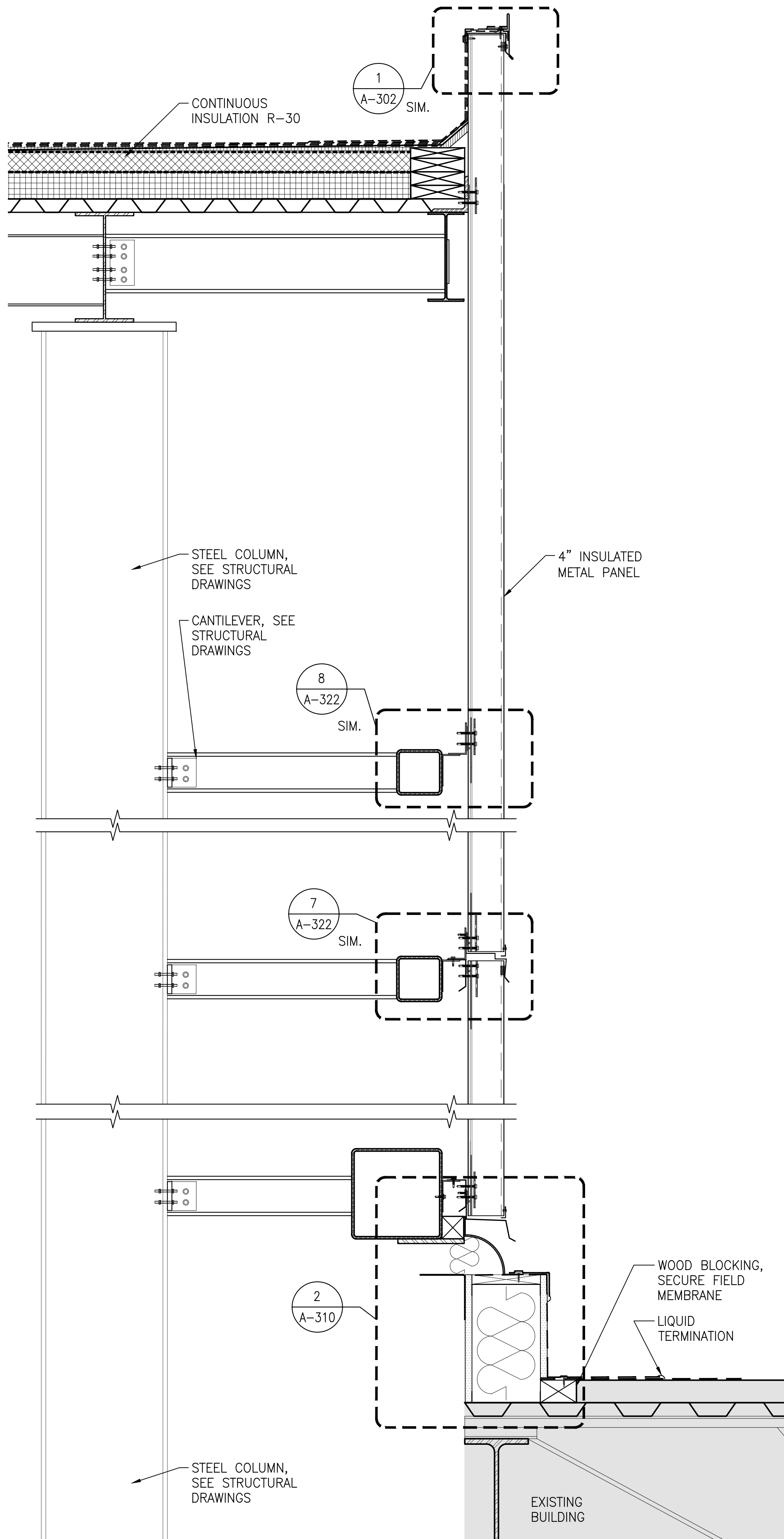
TYP. DETAIL AT AS/RS AND EXISTING BUILDING
