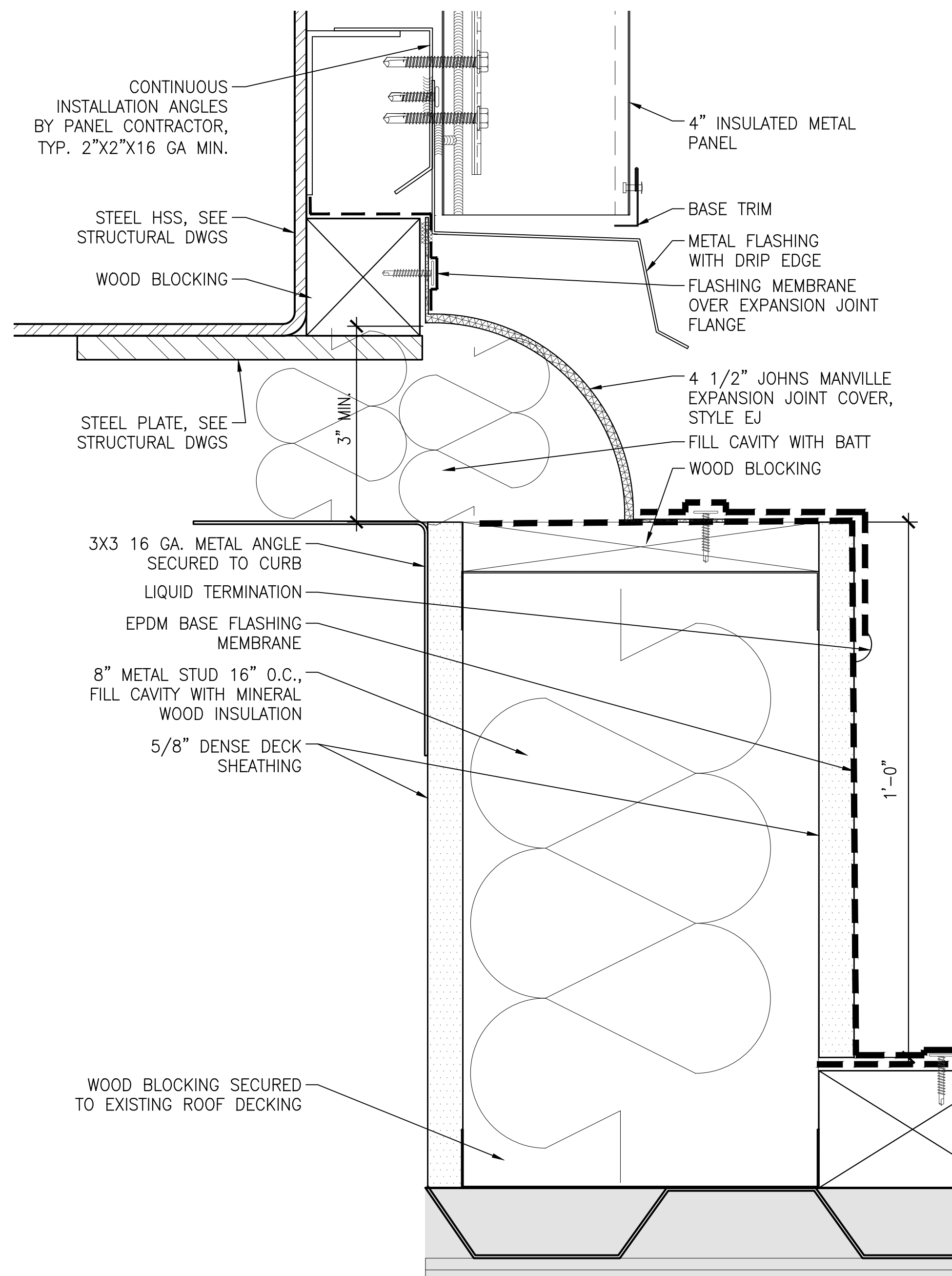
CONNECTION/EXPANSION DETAL
