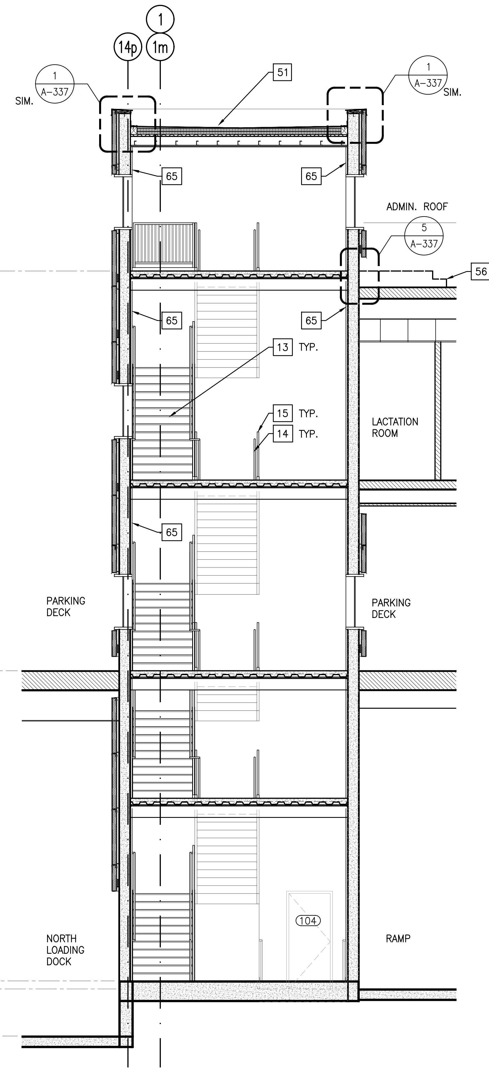
STAIR B - ENLARGED SECTION 2 SCALE: 1/4" = 1'-0"
