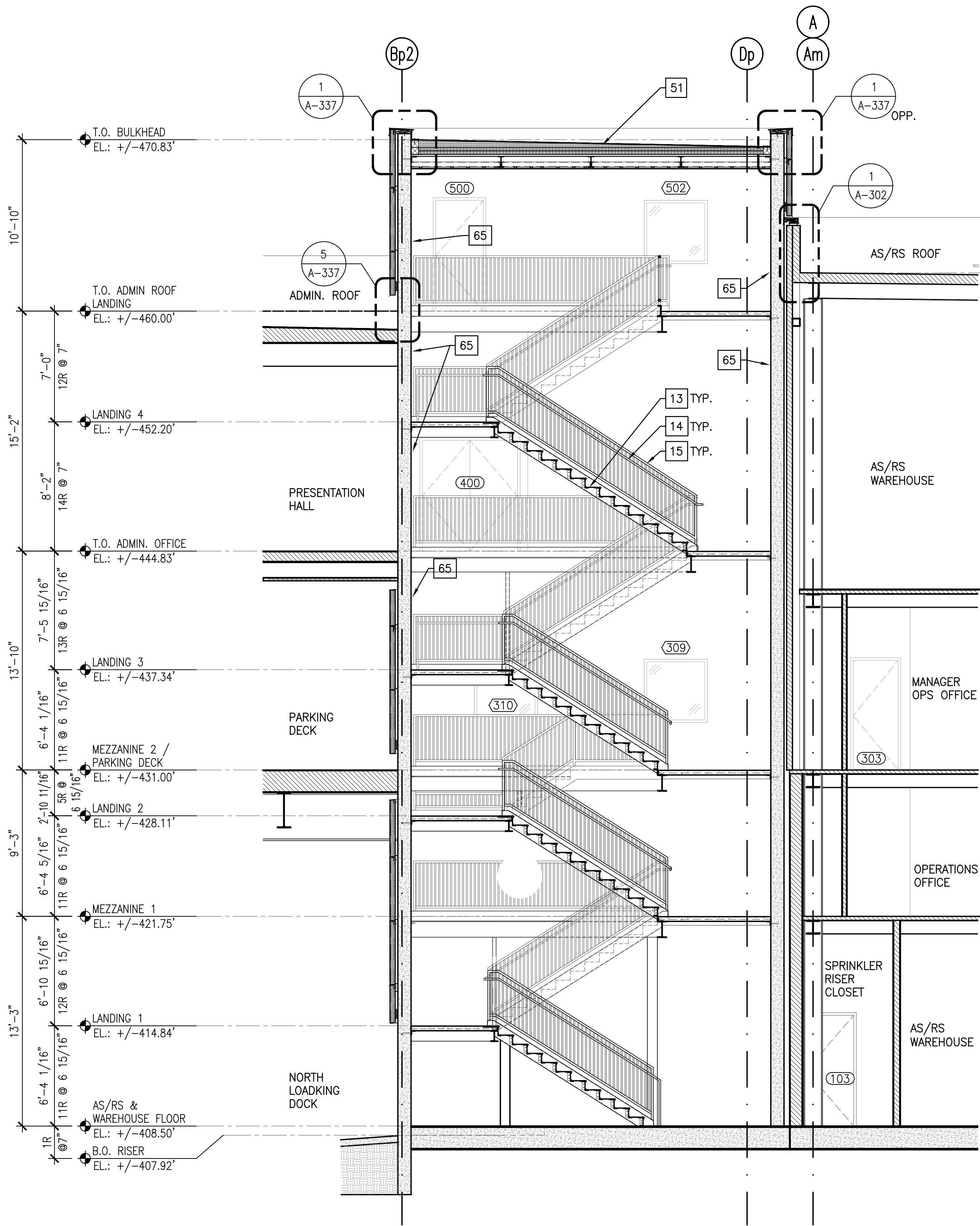
STAIR B - ENLARGED SECTION 1 SCALE: 1/4" = 1'-0"
