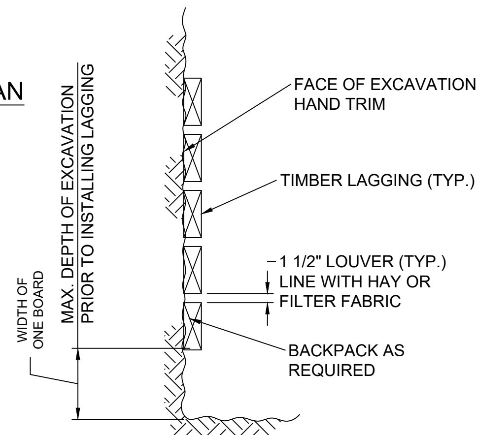
TYPICAL LAGGING INSTALLATION DETAIL SCALE: 3/4" = 1'-0"
