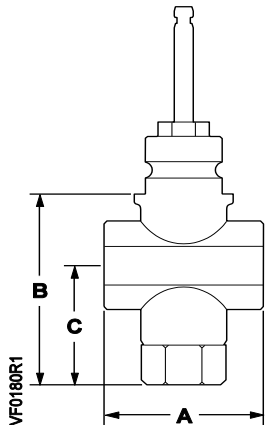
Figure 5. Three-Way Internal Thread NPT x Internal Thread NPT (ITxIT) Valves.
