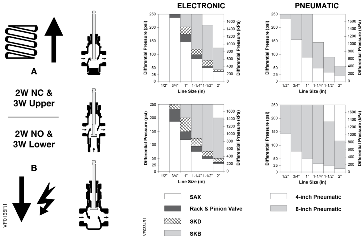
Figure 2. Close-off Pressures.
