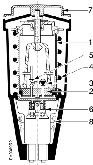
Figure 4. SKD6xU Details.
