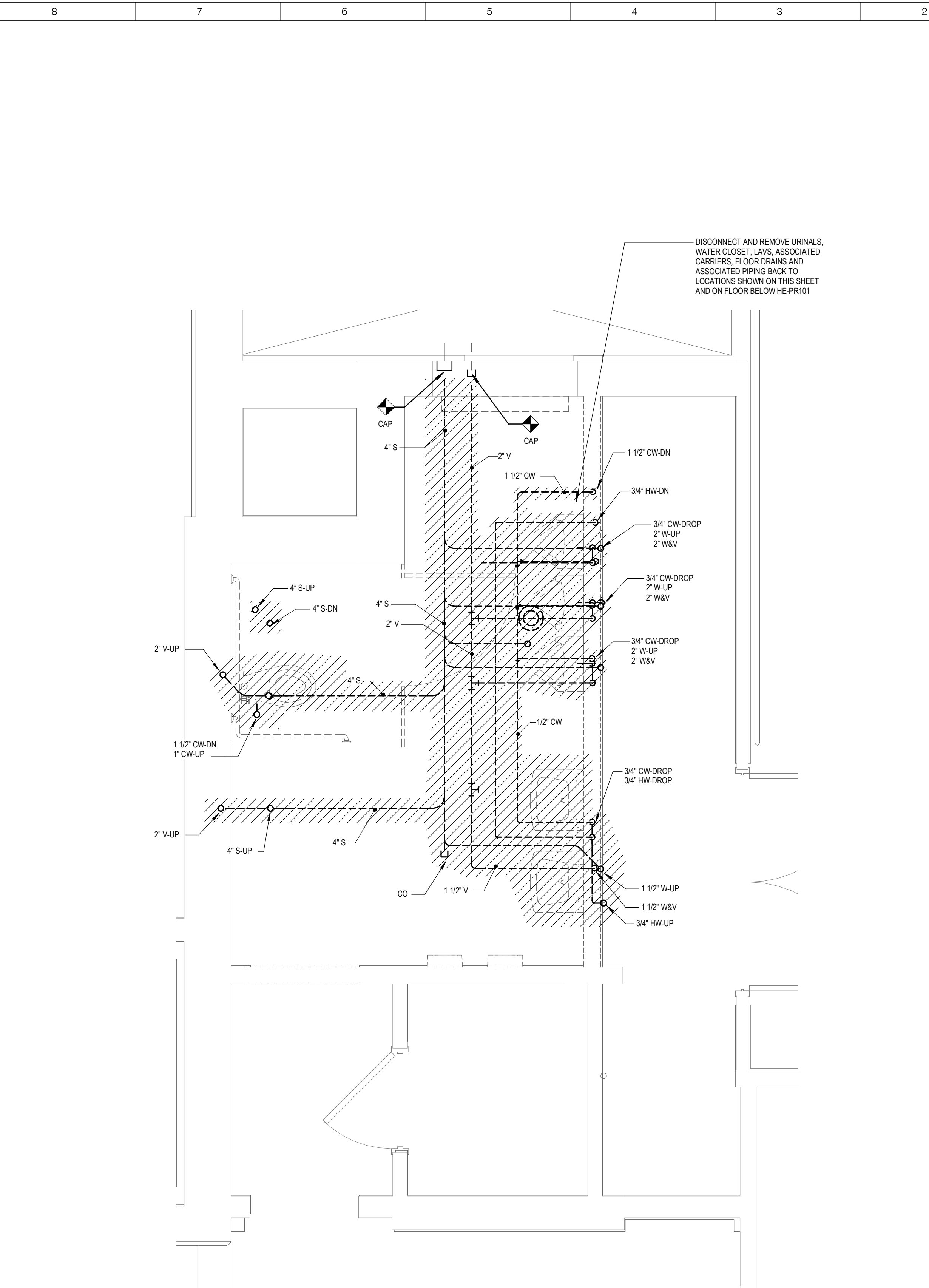
2 FIRST FLOOR BOYS BATHROOM PLUMBING REMOVALS PLAN 1/2" = 1'-0"
